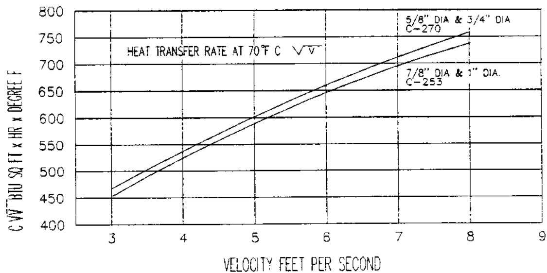
Figure 30 Heat Transfer Through Condenser Tubes
