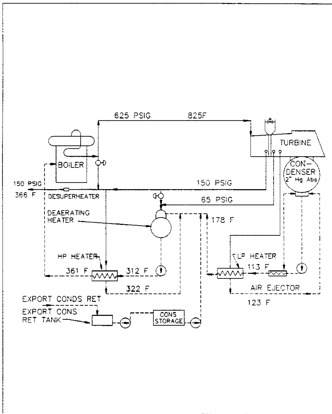
Figure 12 Typical Controlled Extraction - Condensing Cycle
