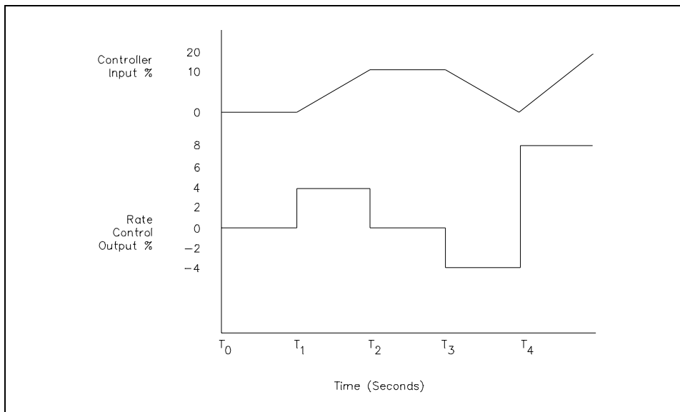
Figure 26 Rate Control Output
