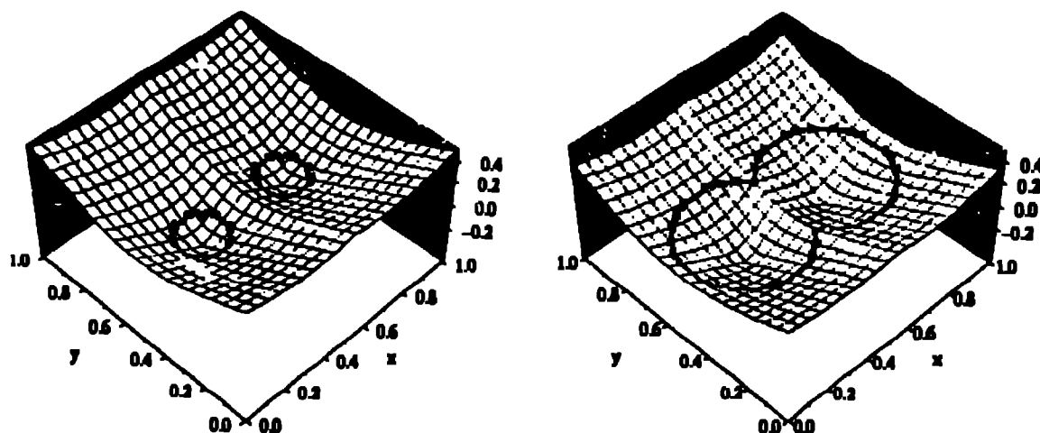
Fig. 3. The level-set function \psi defined initially (as the minimum distance function) and at a later time, for the example of two cylindrically expanding shocks that are at first separated and then merge.
