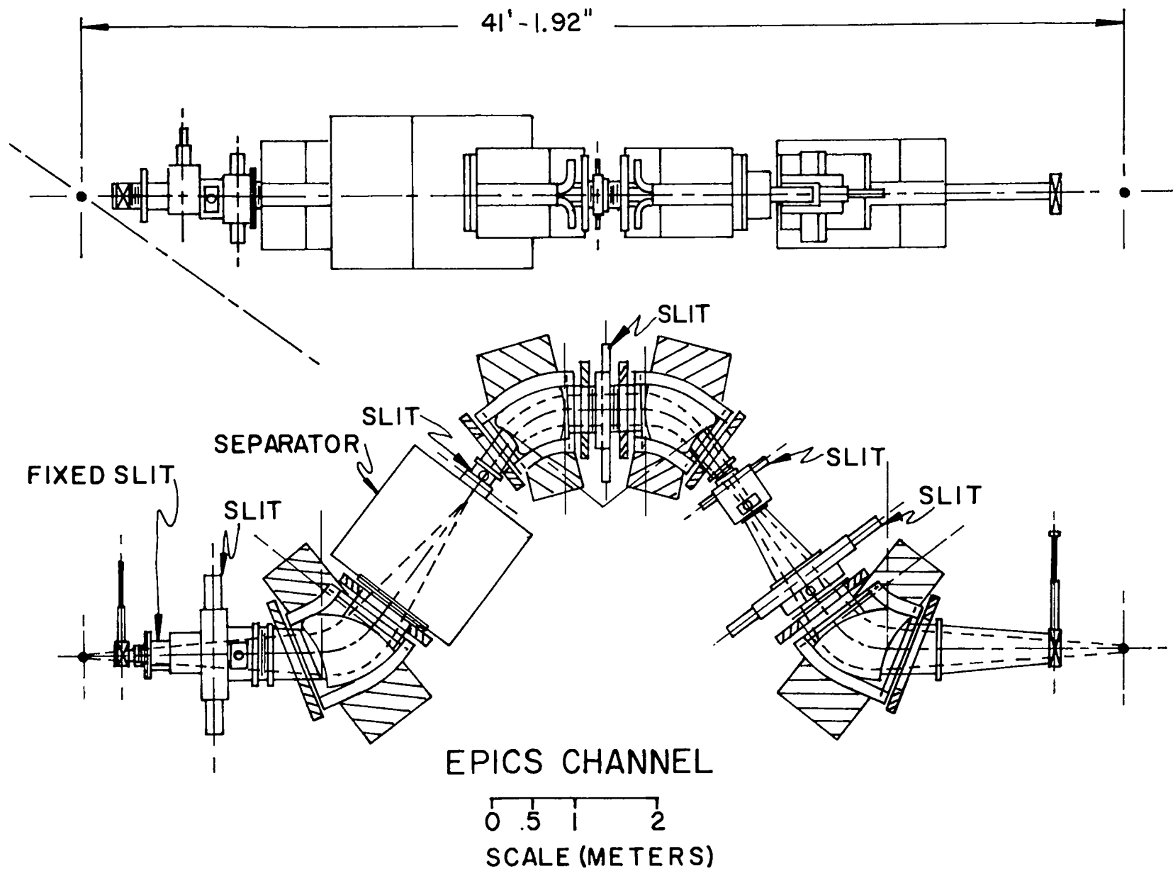
Fig. 16. Energetic Pion Channel (EPICS).
