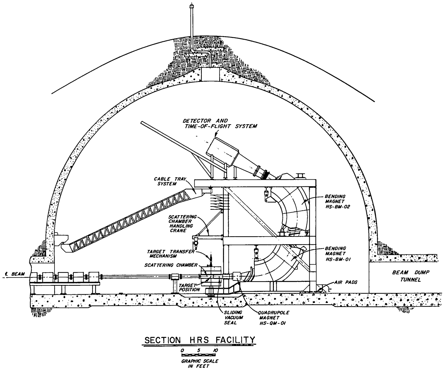
Fig. 21. High-Resolution Spectrometer, elevation (HRS).
