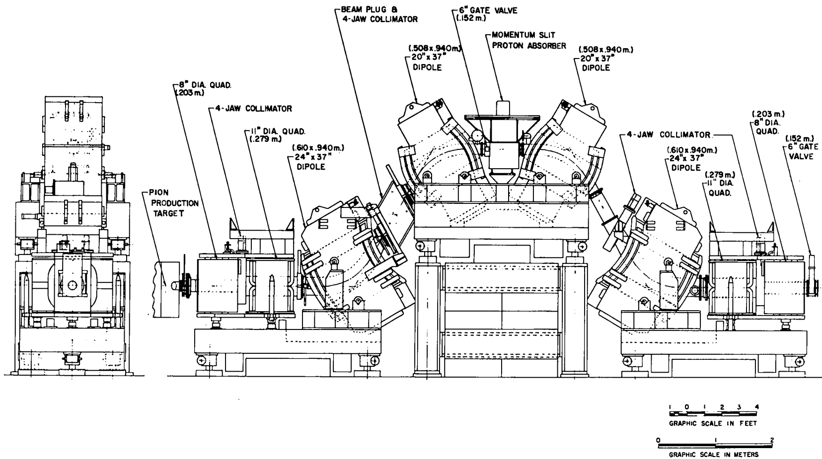
Fig. 15. Low-energy Pion Channel, elevation (LEP).
