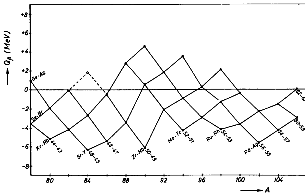
Fig. 11. Way-Wood lines for even-even nuclei.
