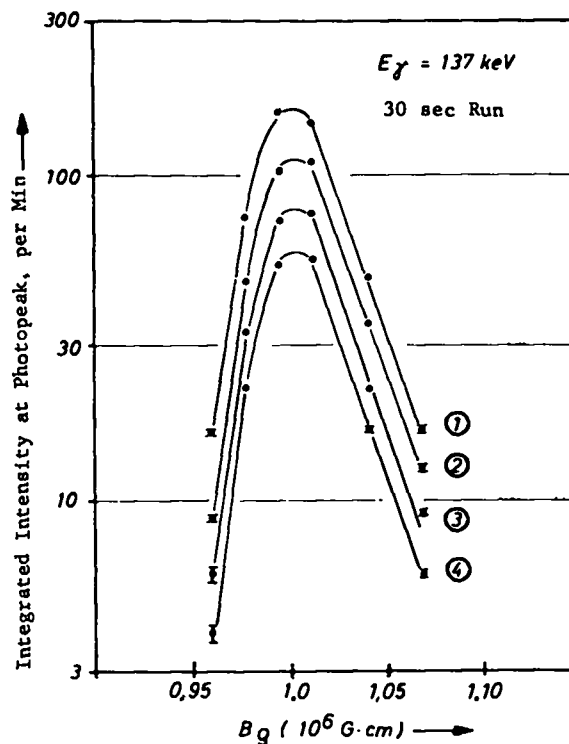
Fig. 5. Example of B_p distribution of a strong \gamma line for the following measuring intervals:
