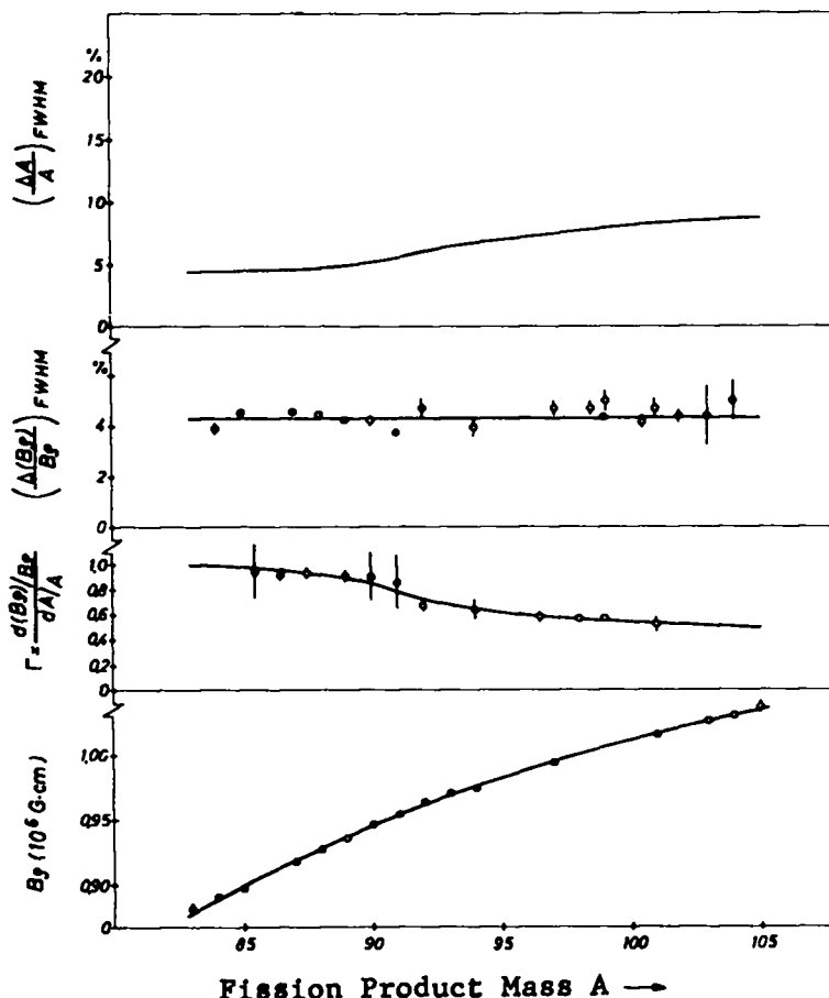
Fig. 6. Mass calibration curve, mass dispersion, B\rho resolution, and mass resolution (bottom to top) for light fission products at 6.5-Torr helium pressure.
