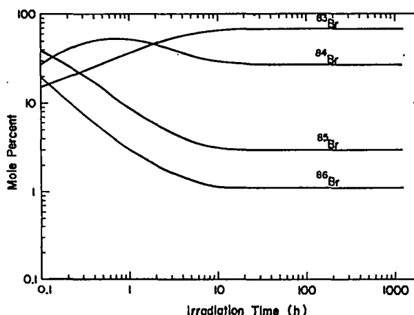
Fig. 463-5. Isotopic concentration of bromine fission products vs irradiation time.
