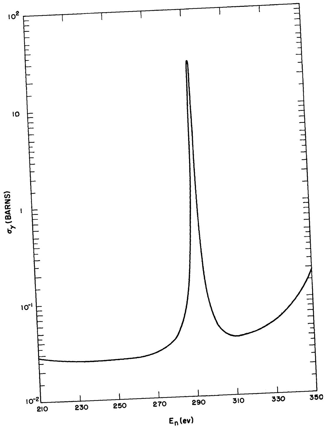
Fig. 6 Molybdenum radiative capture cross section, \sigma_\gamma , versus neutron energy, E_n , from 210 to 350 ev for T = 0.0253 ev.
