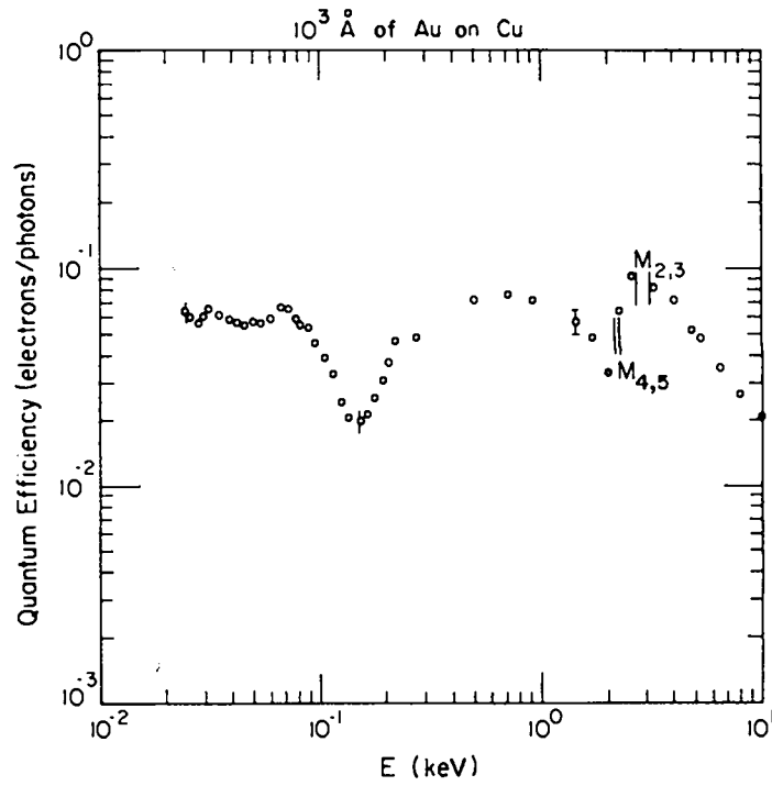
Fig. A-4. Measured quantum efficiency of evaporated gold on copper.
