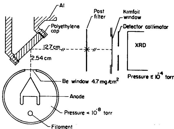
Fig. 11. The LASL fluorescent x-ray source.
