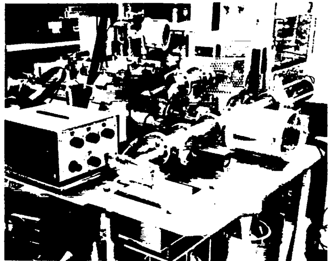
Fig. 12. The LASL fluorescent x-ray source and data acquisition system.
