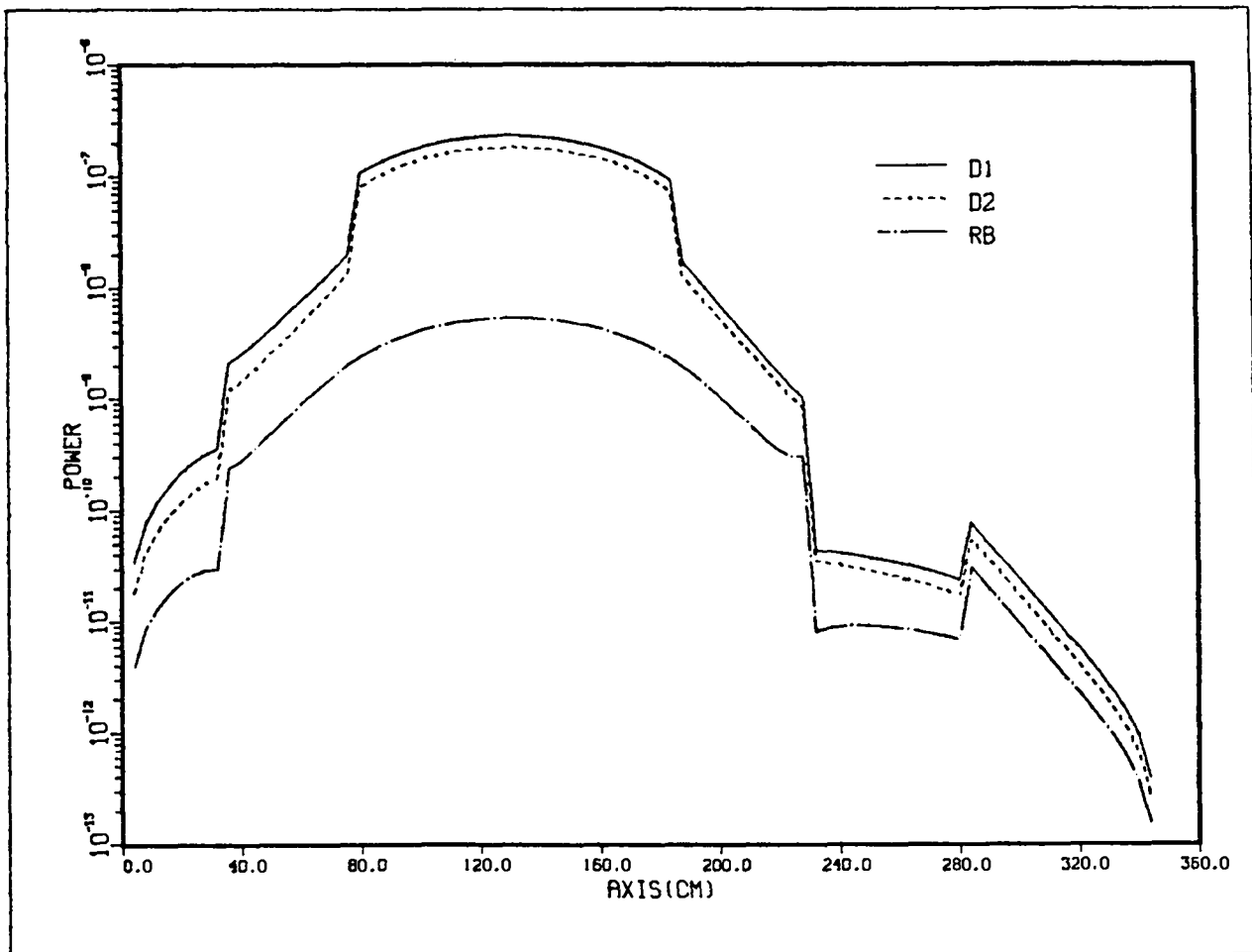
Fig. 60. Axial power traces in two driver regions and radial blanket. Power units normalized to 1 Watt.
