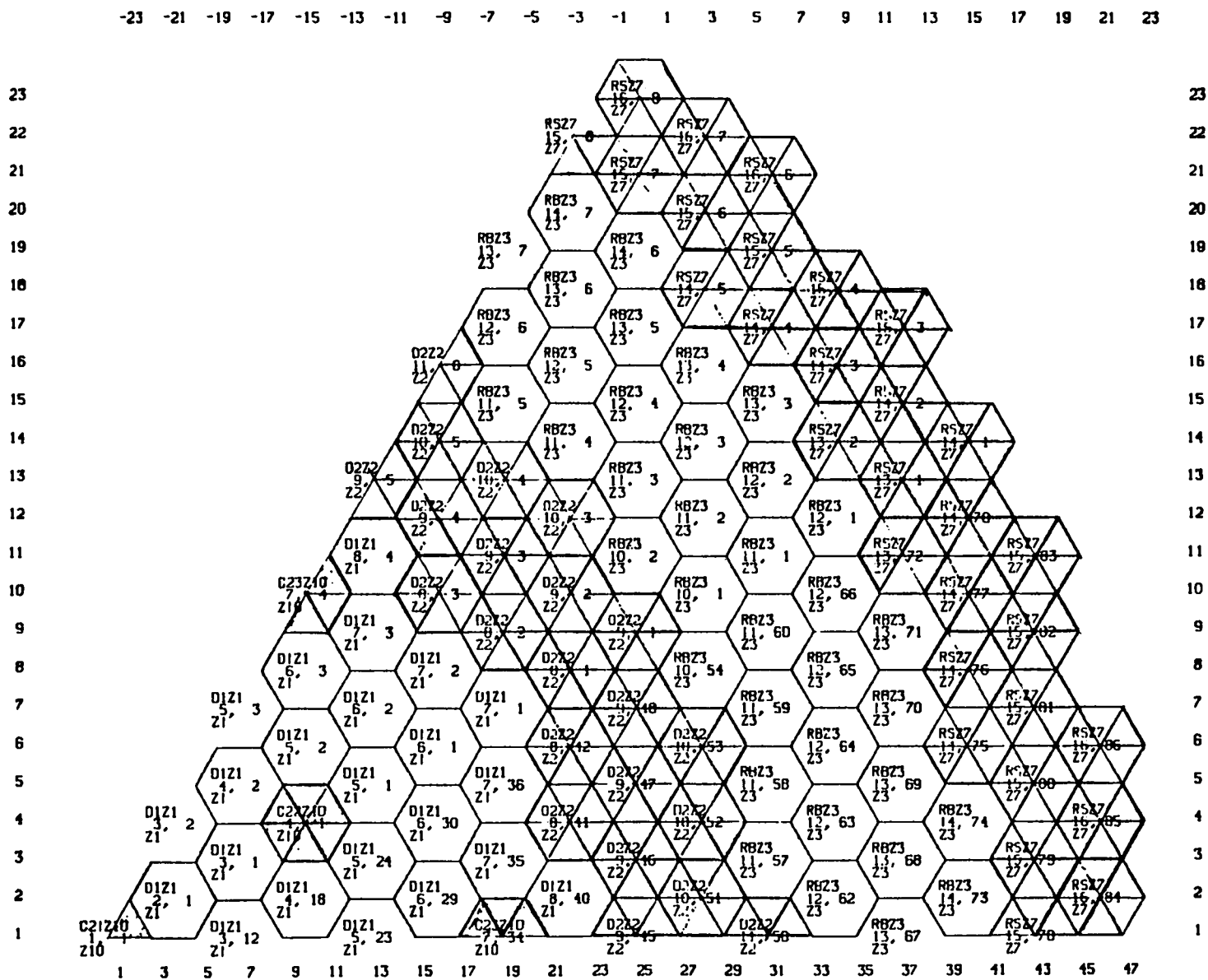
Fig. 59. Mid-plane of CDS Triangular-Z Model.
