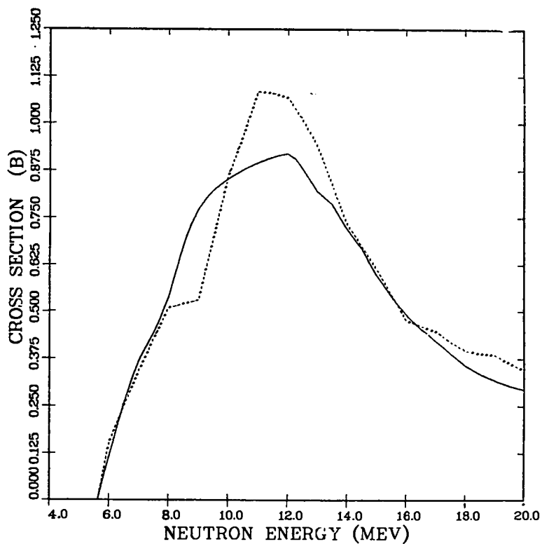
Fig 11. Evaluations of the total gamma-ray production cross sections for neutron reactions on ^{15}\text{N} . See caption to Fig. 10 for explanation of curves.
