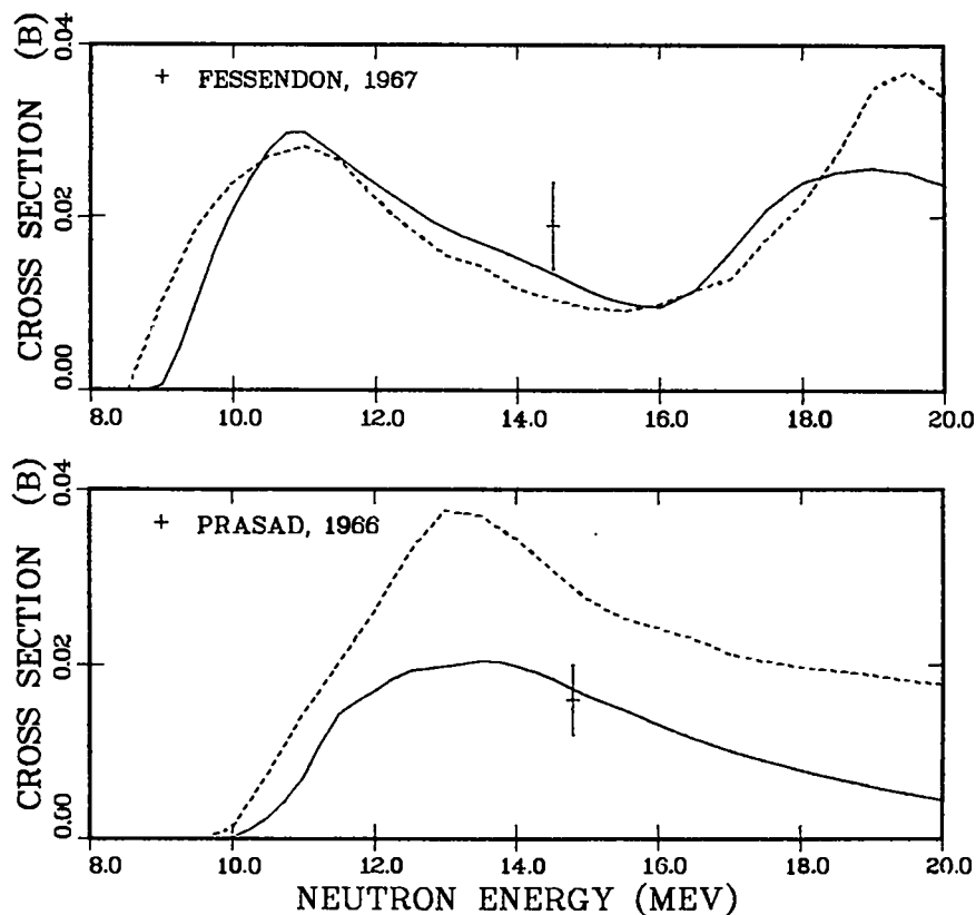
Fig. 10. Measured 22,23 and evaluated cross sections for the ^{15}\text{N}(n,p) [upper] and ^{15}\text{N}(n,d) [lower] reactions from threshold to 20 MeV. The solid curve is the present evaluation, the dashed curve is ENDF/B-V, and the points are experimental data.
