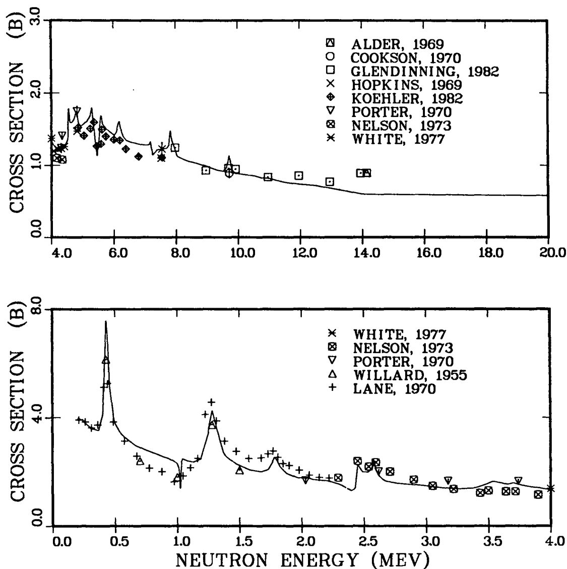
Fig. 32. Elastic neutron cross section for ^{11}\text{B} from 0.2 to 20 MeV.
