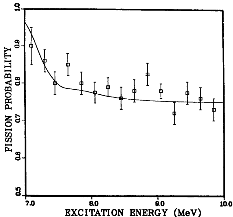
Fig. 15. Our fits to fission probabilities ( P_f ) measured in the ^{238}\text{Np}(^3\text{He},\text{df})\ ^{238}\text{Pu} reaction, which were used f to determine ^{238}\text{Pu} barrier parameters appearing in Table IV, are compared with data.* In these calculations, explicit account was taken of the compound nucleus spin populations produced in this direct reaction.
