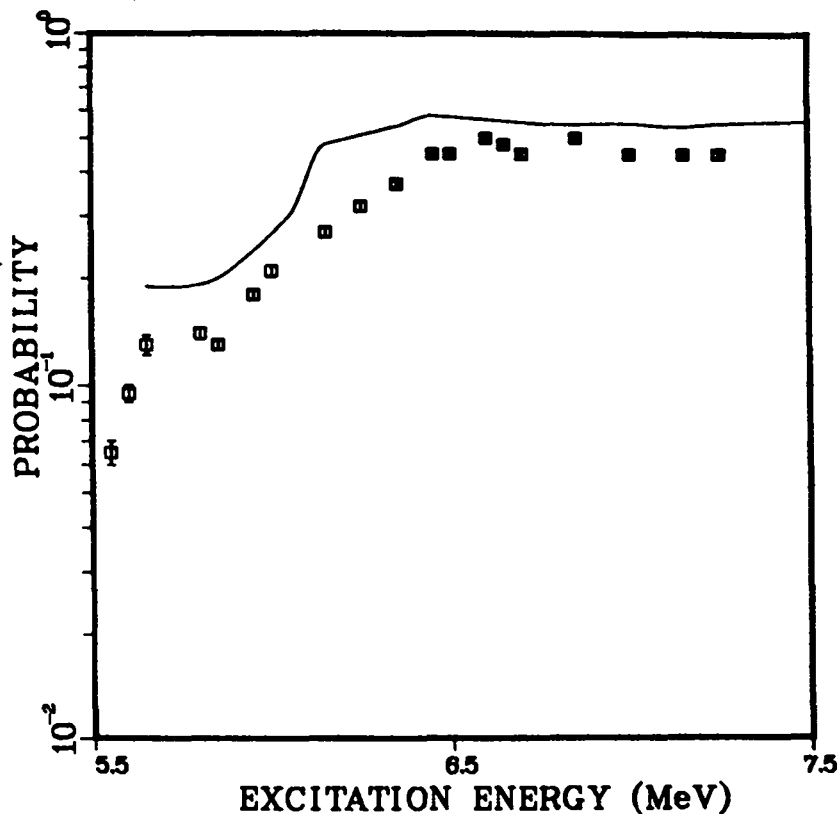
Fig. 14. Fission probabilities (Pf) for ^{239}\text{Pu} measured using the ^{238}\text{Pu}(d,pf)^{239}\text{Pu} direct reaction* are compared with the Pf deduced from new ^{238}\text{Pu}(n,f) measurements 29 (solid curve). The probabilities given by the curve are more consistent with data needed to fit second-chance fission contributions in our n+^{239}\text{Pu} fission calculations.
