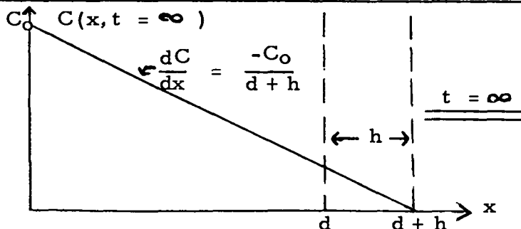
Fig. 2 Steady-State Tritium Distribution
