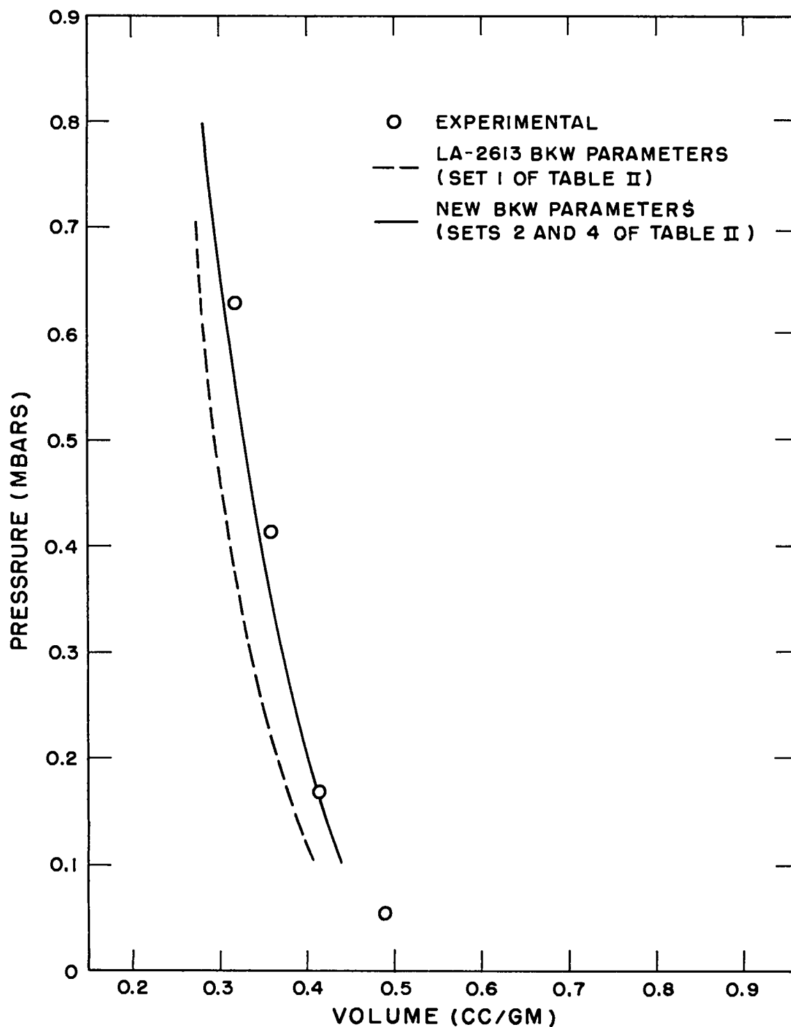
Figure 3. Solid Carbon Dioxide Hugoniot.
