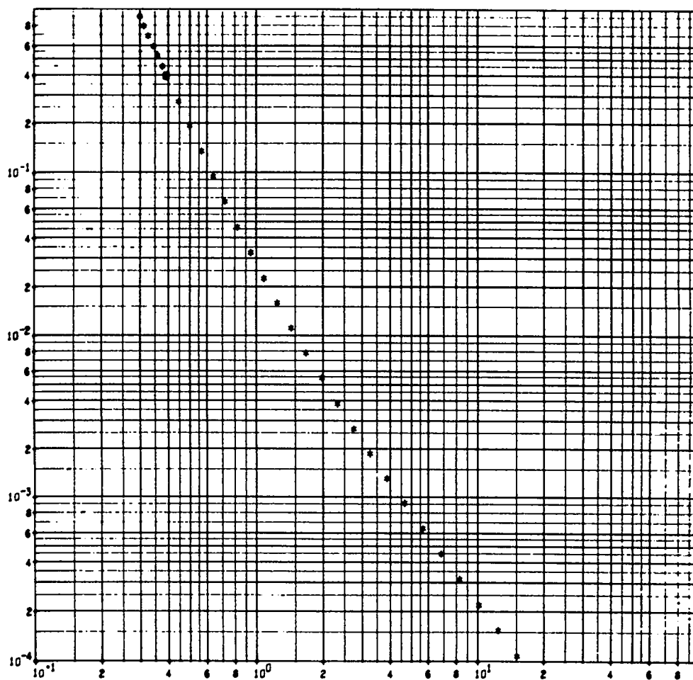
MMX CYCLOTETRAMETHYLENE TETRANITRAMINE PRESSURE-VOLUME ISENTROPE THRU THE C-J VALUE
