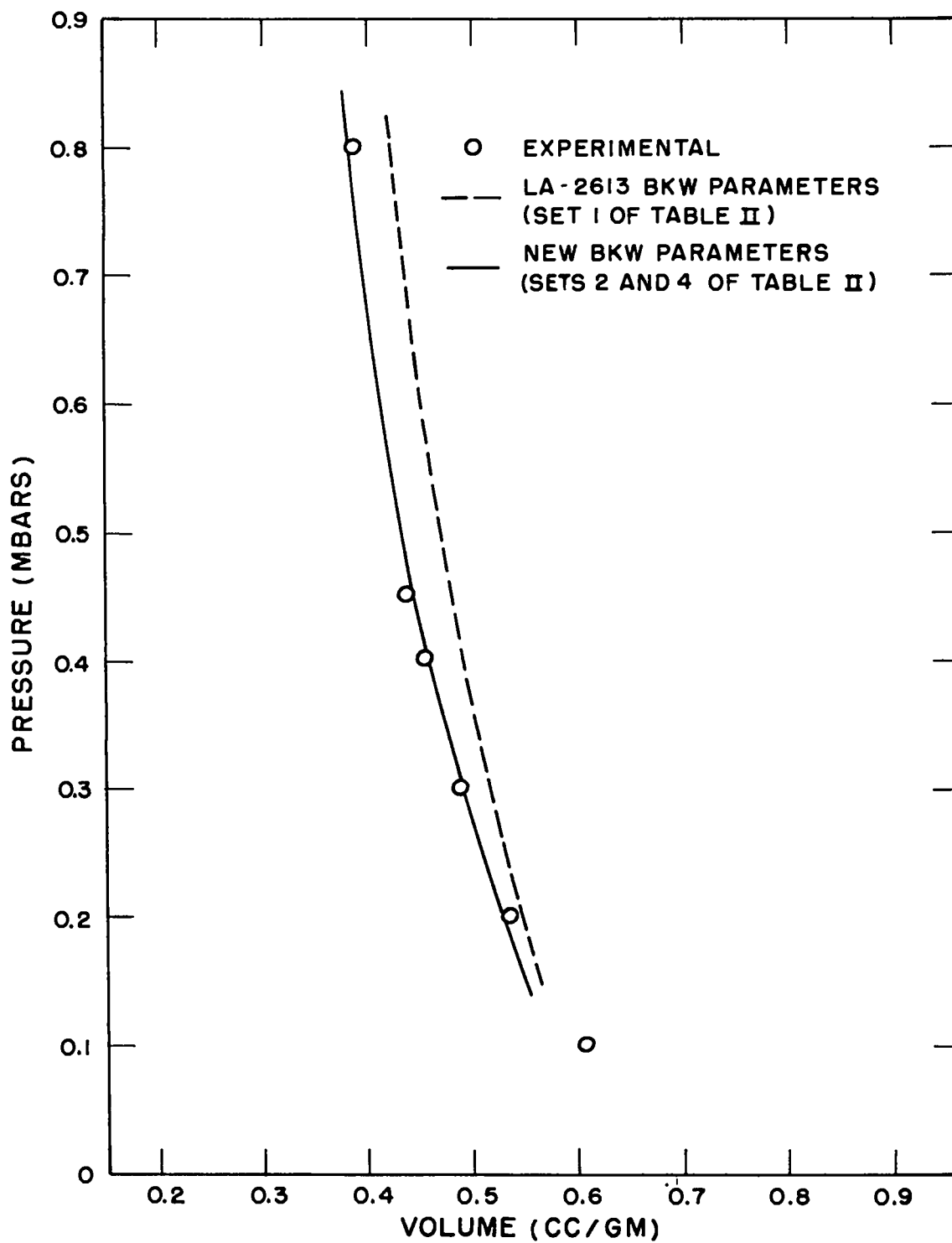
Figure 1. Water Hugoniot.
