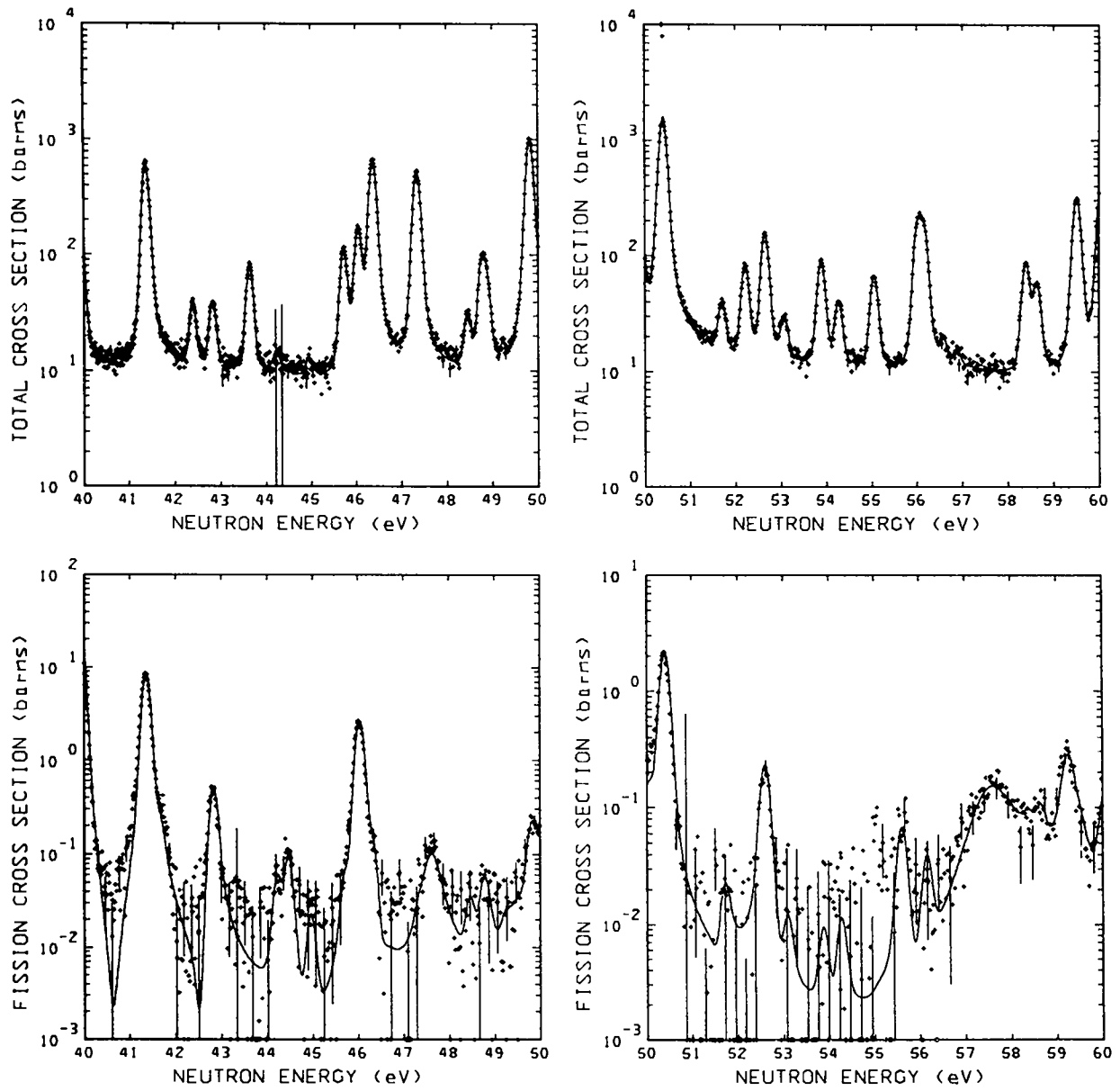
Fig. 3. Total and fission cross sections from 40 to 60 eV. The statistical errors are represented by vertical lines.
