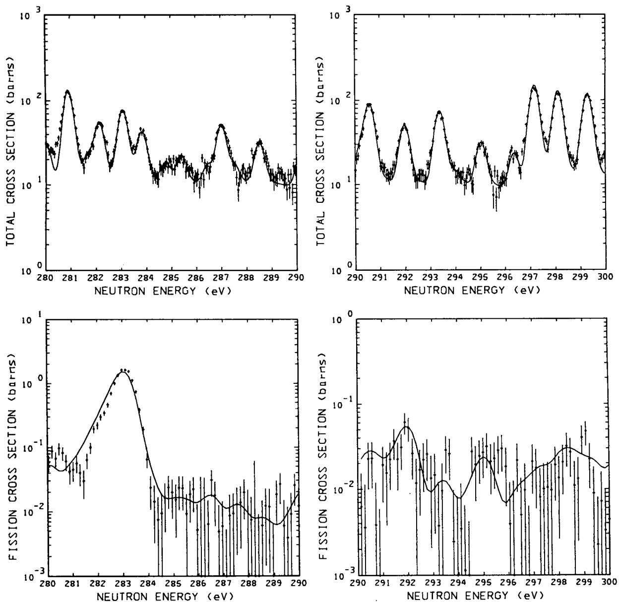
Fig. 15. Total and fission cross sections from 280 to 300 eV. The statistical errors are represented by vertical lines.
