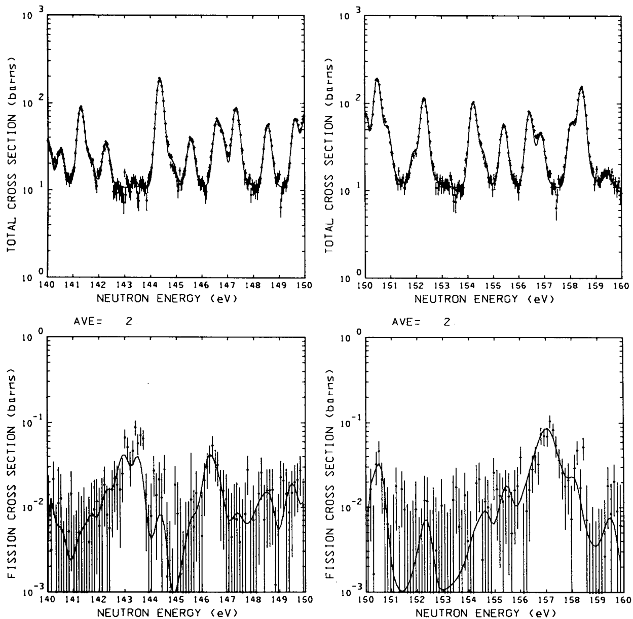
Fig. 8. Total and fission cross sections from 140 to 160 eV. AVE represents the number of points averaged. The statistical errors are represented by vertical lines.
