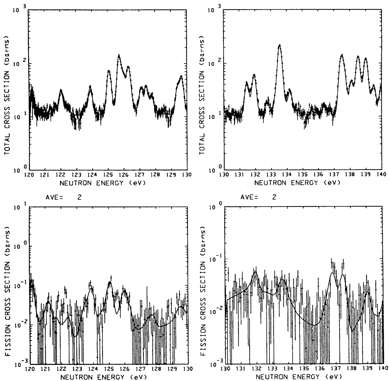
Fig. 7. Total and fission cross sections from 120 to 140 eV. AVE represents the number of points averaged. The statistical errors are represented by vertical lines.
