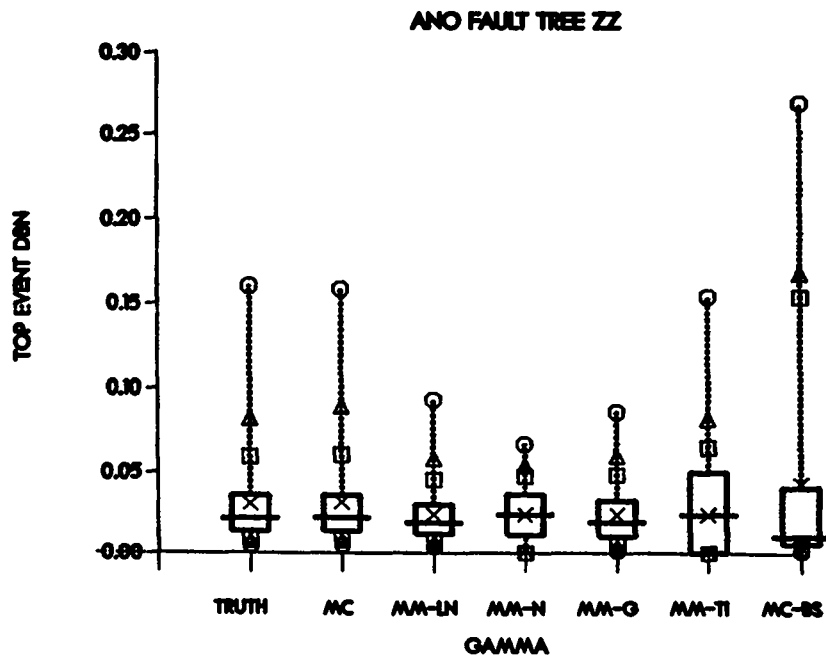
Fig. 36. Comparative performance of the methods for fault tree ZZ and gamma basic event distributions.
