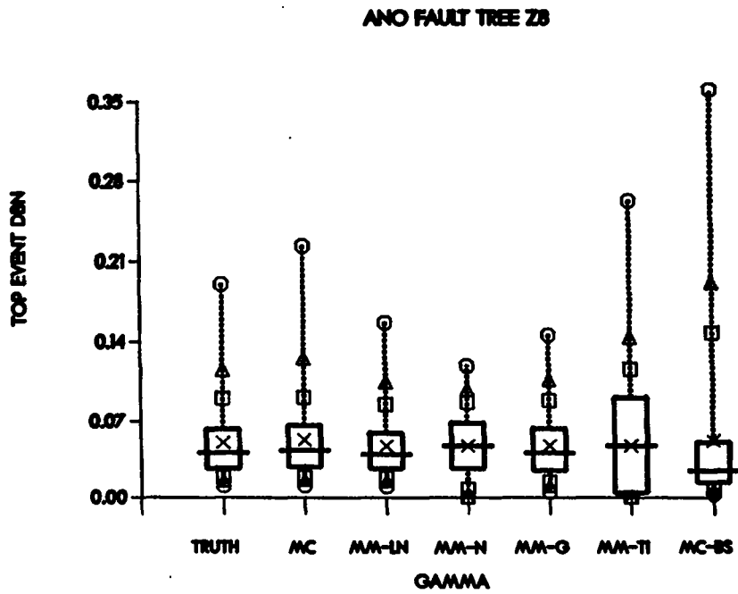
Fig. 35. Comparative performance of the methods for fault tree Z8 and gamma basic event distributions.
