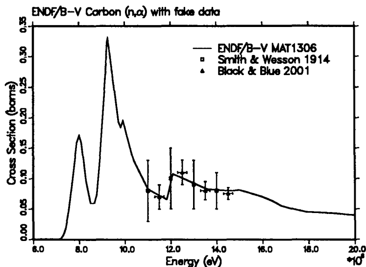
Figure 7: Carbon (n,α) cross section compared with two sets of simulated experimental data represented with two types of error bars.
