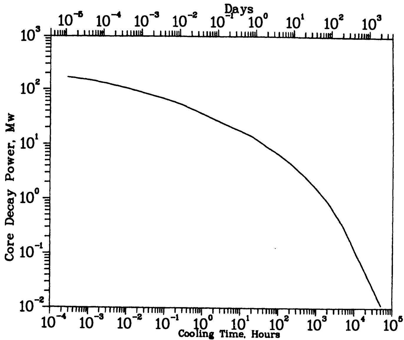
Fig. 2. Total core decay power from actinides and fission products, Three Mile Island, Unit 2.
