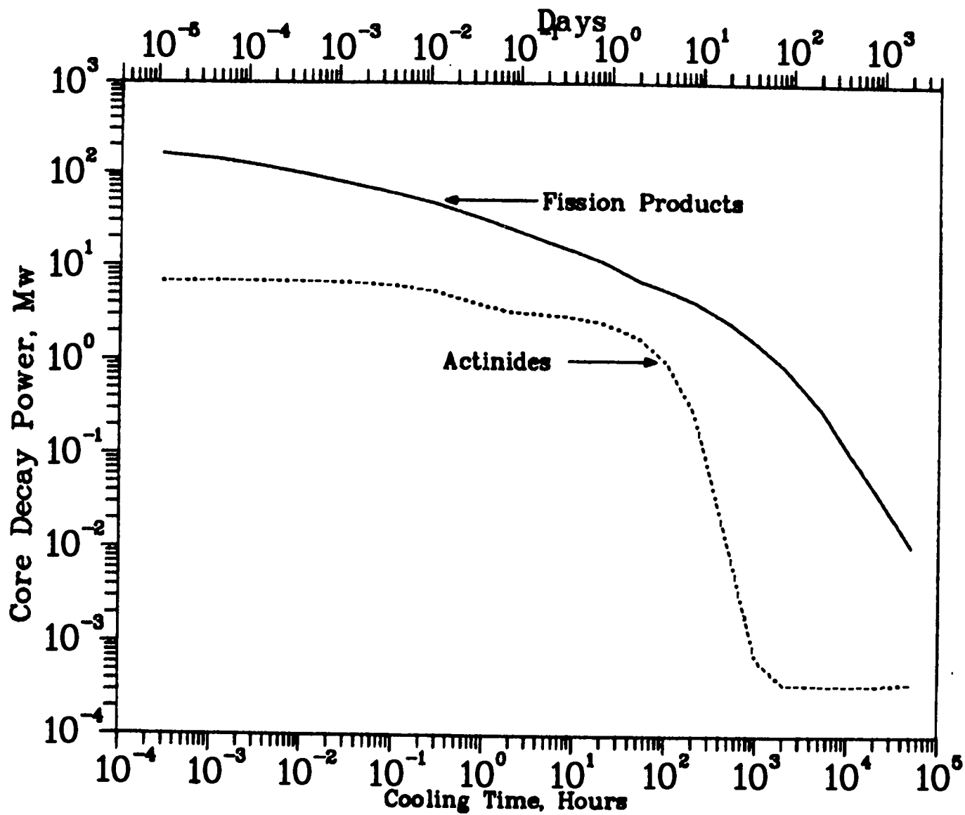
Fig. 3. Actinide and fission-product decay power components, Three Mile Island, Unit 2.
