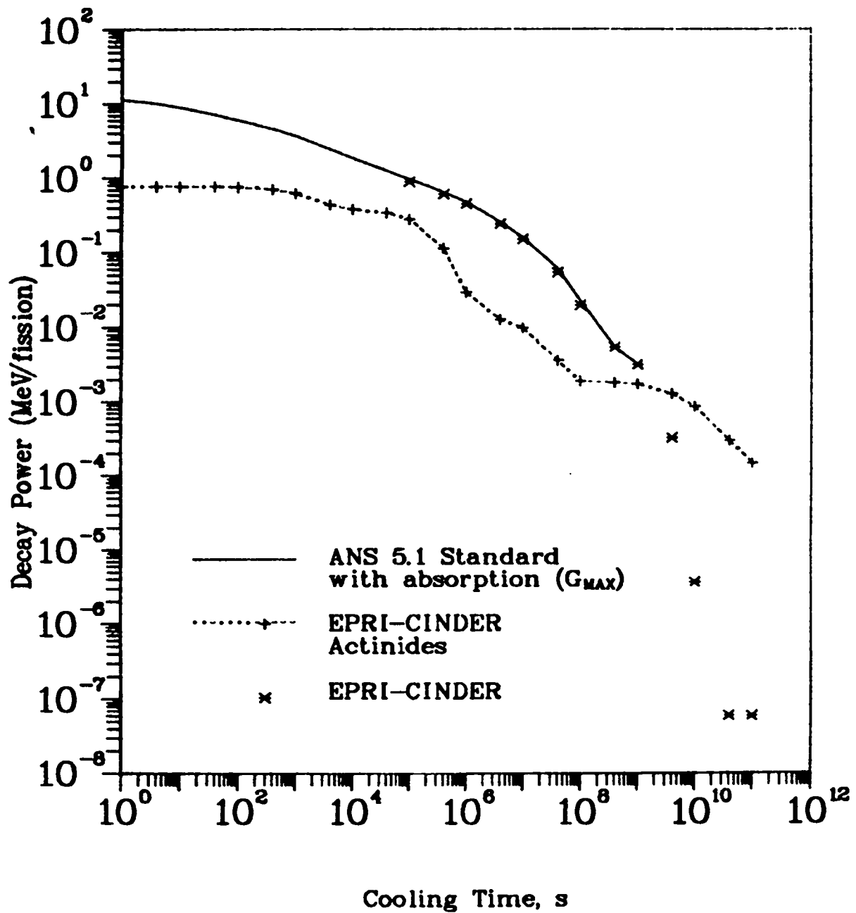
Fig. E-5. Fission-product and actinide decay power, case 1A, PWR, 2.56% U235/U238 fuel, 34 GWD/MT, 1082 days.
