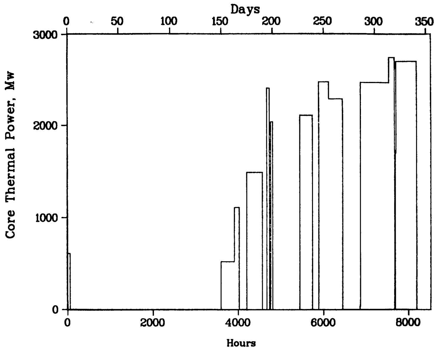
Fig. 1. CINDER Histogram core power history. Three Mile Island, Unit 2.
