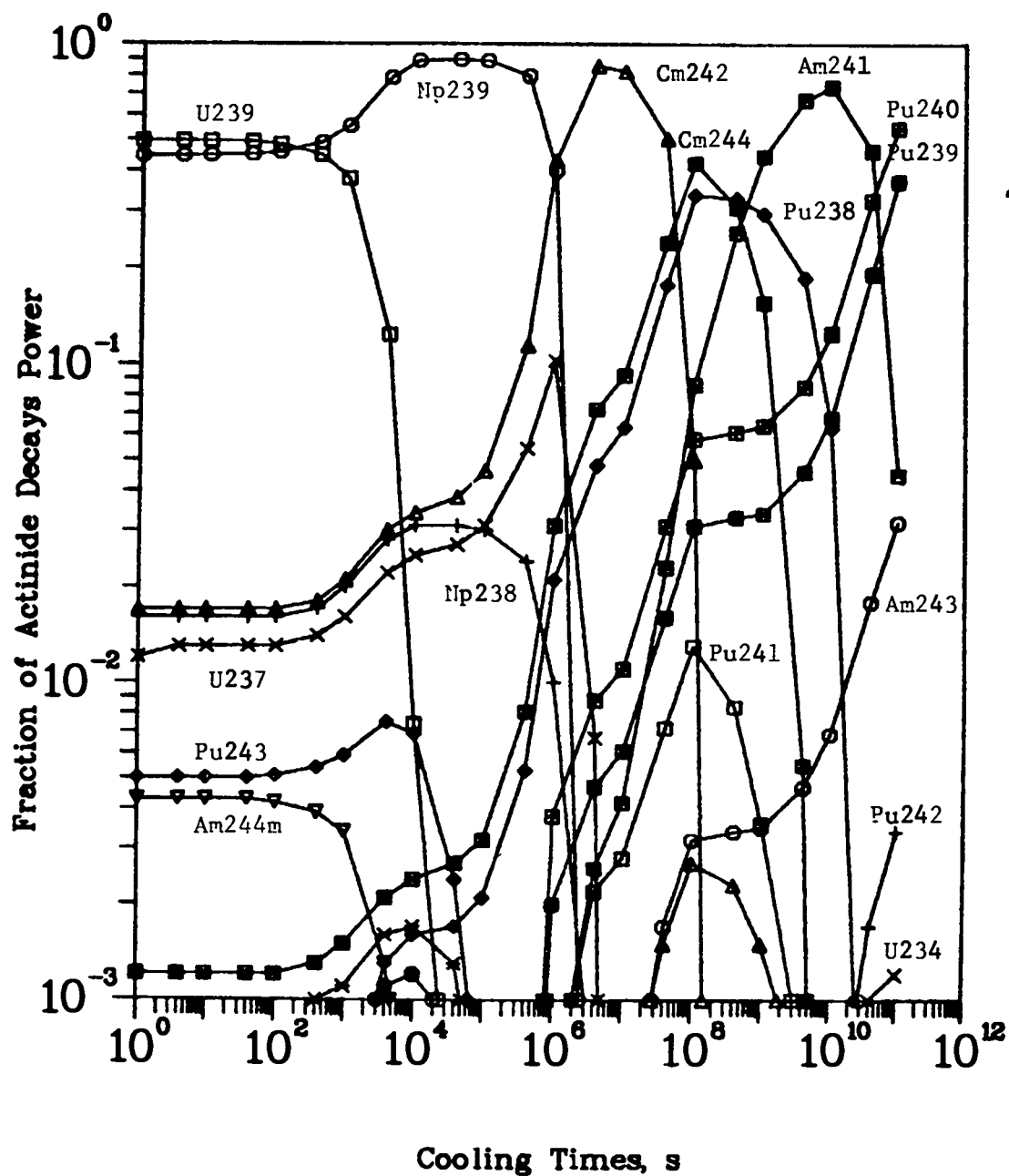
Fig. E-4. Nuclide contributors to actinide decay power, case 1A, PWR, 2.56% U235/U238 fuel, 34 GWD/MT, 1082 days.
