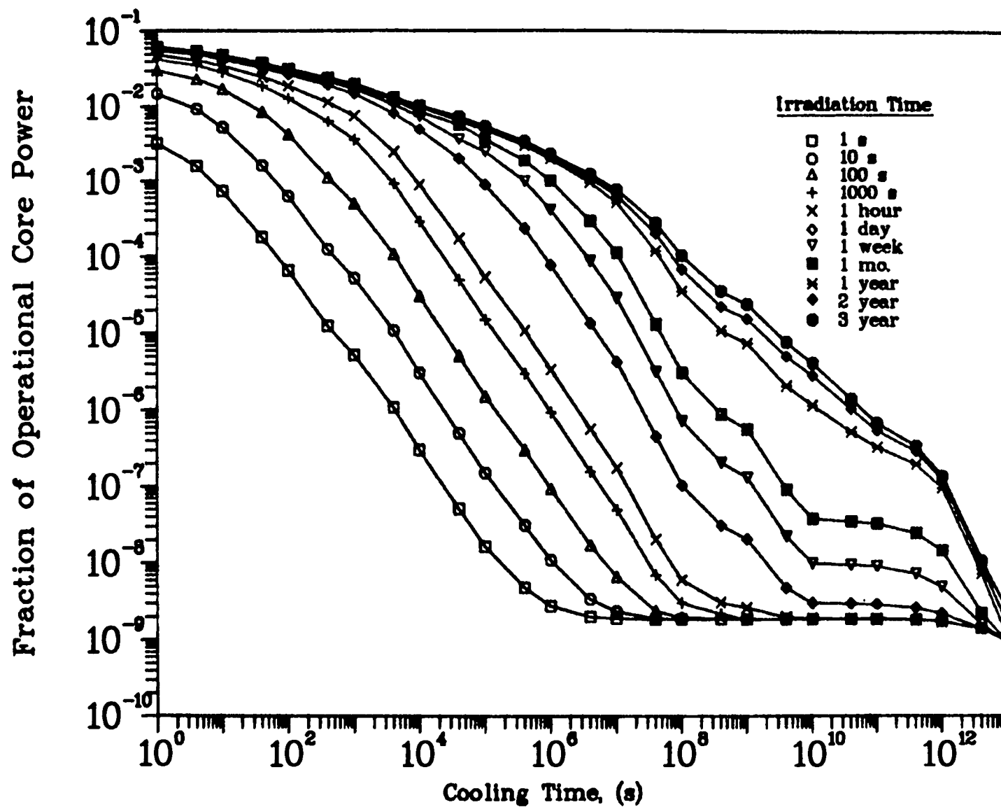
Fig. 5. Total (fission-product plus actinide) decay power fraction of operational core power vs cooling time.
