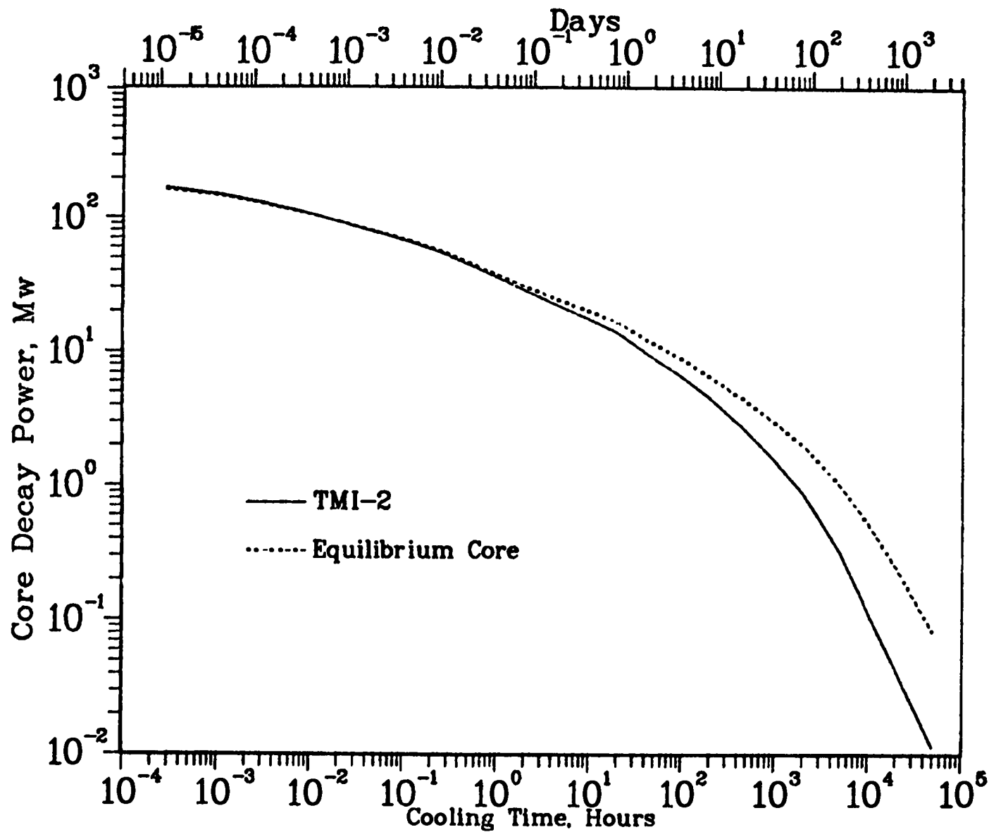
Fig. 4. Comparison of calculated decay power of TMI-2 with end-of-cycle equilibrium core.
