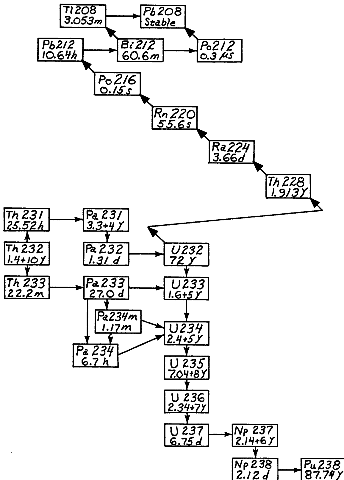
Fig. E-13. Actinide nuclides important to decay power in \text{U}^{233}/\text{Th}^{232} -fueled light water reactors.
