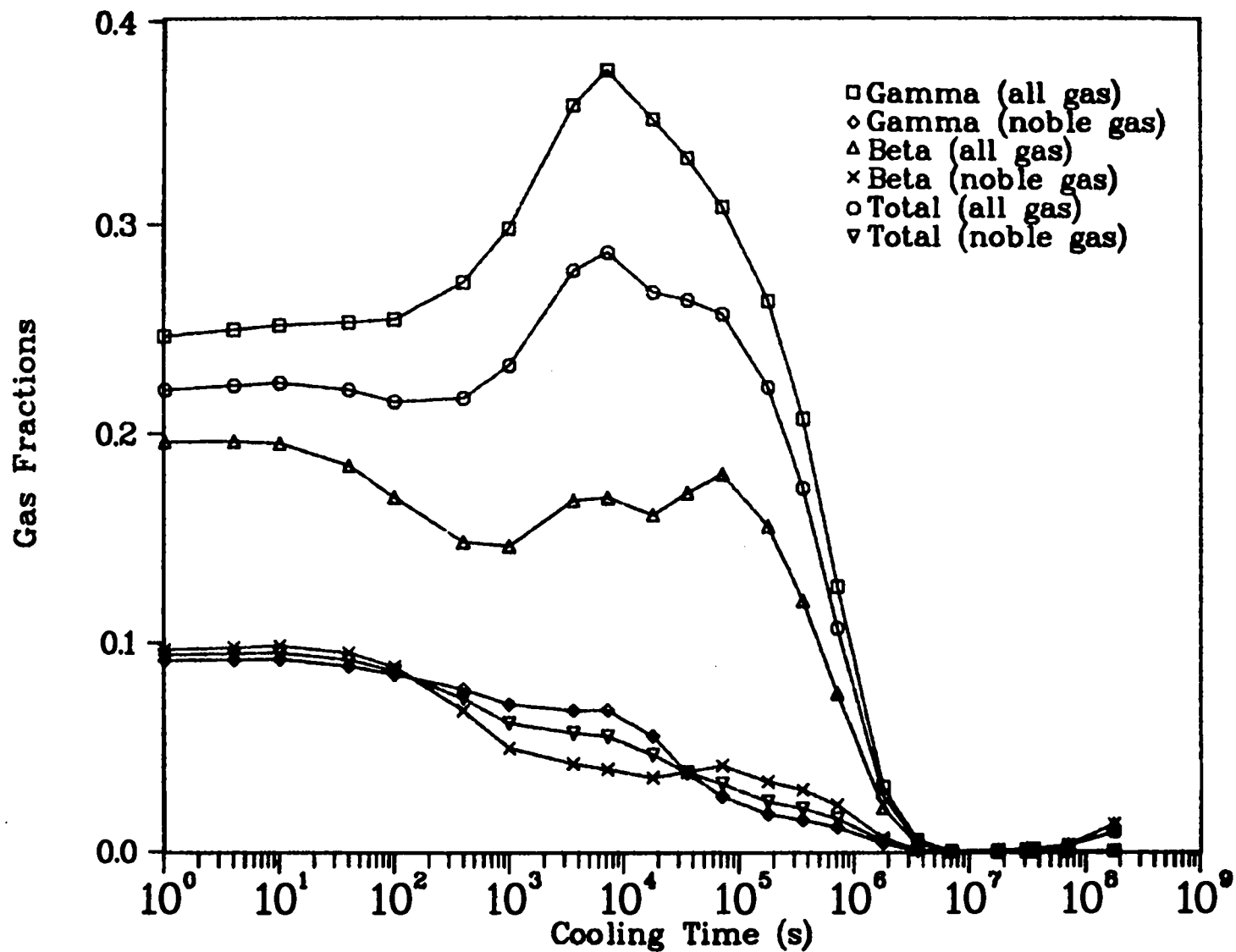
Fig. C-1. TMI-2 gas fraction of total fission-product decay power.
