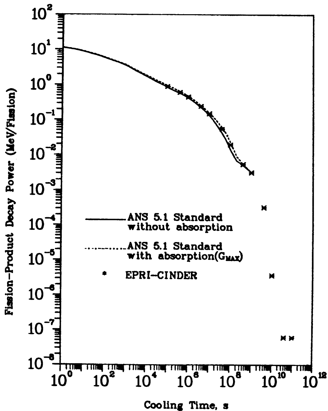
Fig. E-2. Fission-product decay power, case 1A, PWR, 2.56% U235/U238 fuel, 34 GWD/MT. 1082 days.
