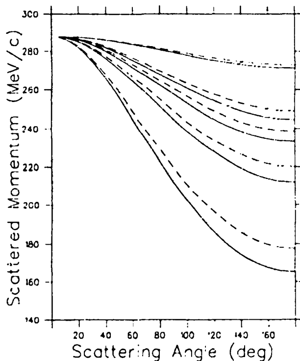
Figure 2.19: The momentum of scattered particles from various targets, from top: Carbon, {}^4\text{He} , Tritium, Deuterium, Hydrogen. The channel is tuned for 180 MeV pions, which corresponds to \sim 287.5 MeV/c momentum for all particles. Towards back angles, there is a very wide divergence in the scattered momentum. Electrons (dashed lines) and pions (solid lines) have about the same scattering kinematics.
