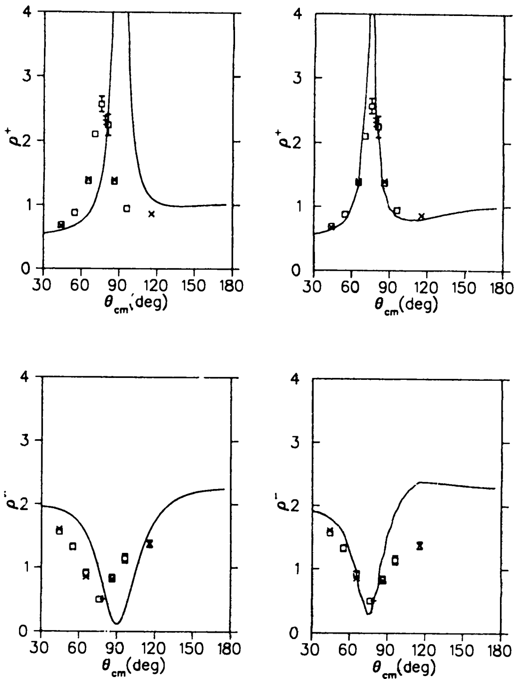
Figure 1.13: \rho^+ and \rho^- , using sum-of-gaussian for factors from [Bar85] and a single-scattering impulse approximation. left: p-wave-only amplitudes. right: VPI-phase-shift amplitudes.
