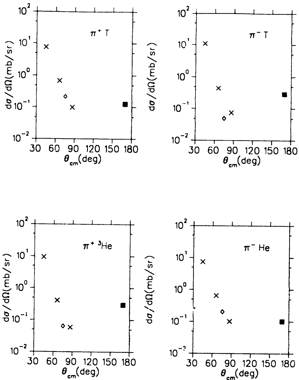
Figure 4.10: Cross sections at 220 MeV. x Exp. 905 [Pil91], ◇ Exp. 1032 [Pil92] [Ber91], filled square current experiments.
