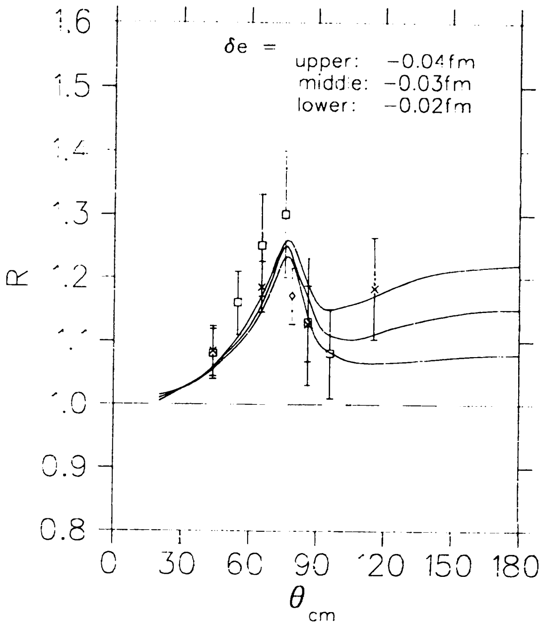
Figure 1.16: R from Gibbs and Gibson[Gib91]. The three curves show the effects of varying \delta_e by \pm 0.01 \text{ fm} , assuming \lambda_e = 0.035 \text{ fm} . \square Exp. 546 [Nef90], \times Exp. 905 [Pil91], \diamond Exp. 1032 [Pil92] and [Ber91].
