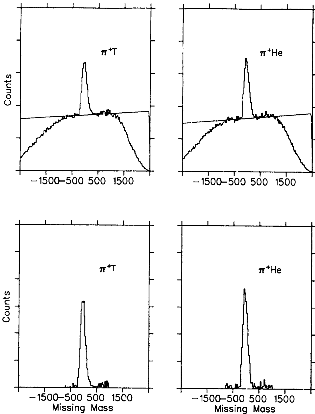
Figure 3.12: Example of the line subtraction technique for 155^\circ , upper left, \pi^+T and line background. Lower left, \pi^+T with background line subtracted. Upper right, \pi^+{}^3He and line background. Lower right, \pi^+{}^3He with line background subtracted.
