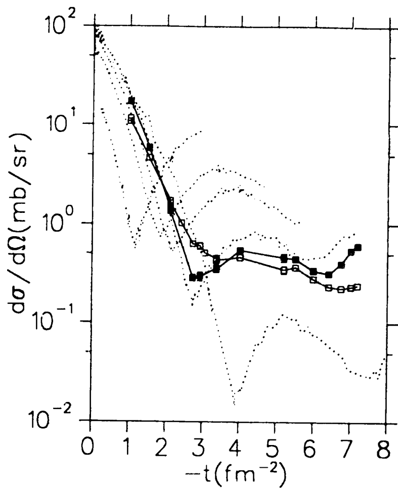
Figure 4.7: Dotted : \pi^+{}^4\text{He} scattering at 90, 130, 150, 180 and 240 MeV, from top to bottom. Filled squares : \pi^-T at 180 MeV. Open squares : \pi^+T at 180 MeV. The dotted lines connect data points from [Bri91], but the actual points are not shown.
