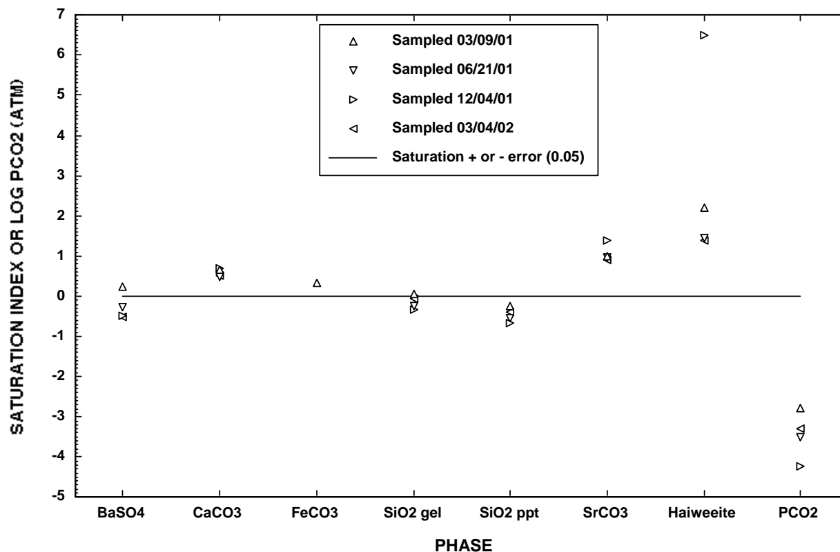
Figure 6.3-2. Results of saturation index calculations using MINTEQA2 for well R-22 (regional aquifer, 1273.5 ft)
