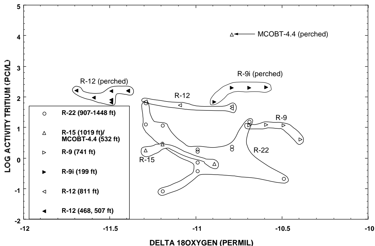
Figure 5.1-10. Delta ^{18}\text{O} (permil) versus log activity tritium (pCi/L) for wells R-9, R-9i, R-12, R-15, R-22, and MCOBT-4.4
