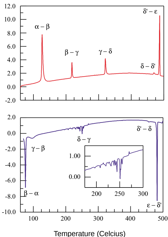
These graphs show heat flow as a function of temperature for pure plutonium. The top graph shows the heating curve; the bottom graph shows the cooling curve.
