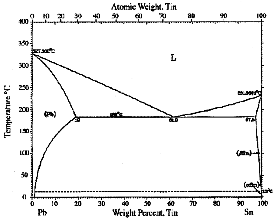
Figure 1a. Equilibrium phase diagram of the Sn-Pb binary alloy.
