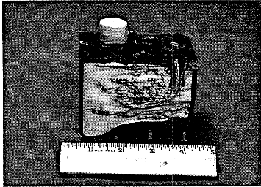
Figure 24. (Continued). Segment of the MC1814 unit after water jet cutting which contains the targeted circuit boards: (a) First cut from the unit to separate the segment of interest. Segment of interest in (b) the front view and (c) rear view. In the front view (b), the numbers refer to the circuit boards in positions noted in Figure 22b.
