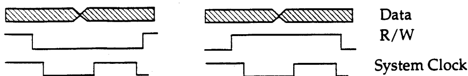
Figure .B Writing Data
