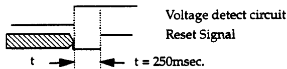
Figure 5. Reset Timing
