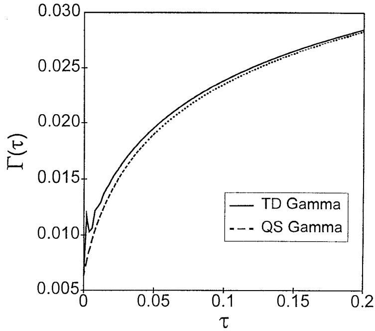
Figure 3. Time variation of electron energy comparing the time-dependent and quasistatic models for the conditions of Fig. 2.
