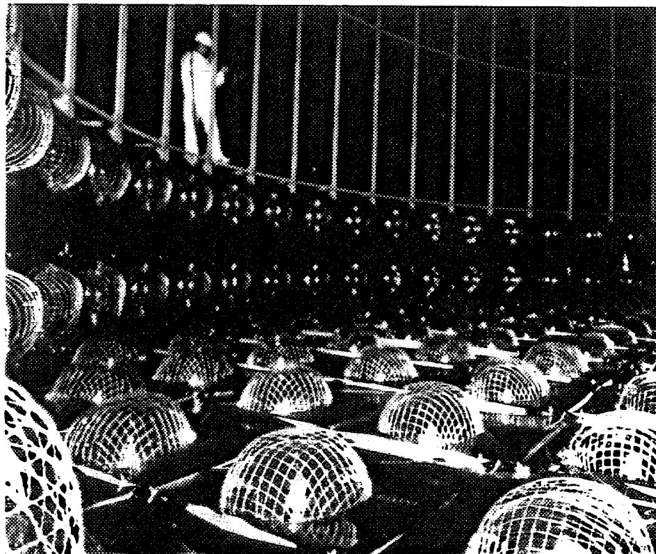
Fig. 3. Photograph of the Kamioka nucleon-decay detector under construction at a depth of 2700 mwe in a lead-zinc mine about 300 kilometers west of Tokyo. Already installed are the bottom layer of photomultipliers and two ranks of photomultipliers on the sides of the cylindrical volume. The wire guards around the photomultipliers protect the workers from occasional implosions. The upper ranks and top layer of photomultipliers were installed from rafts as the water level was increased. The detector contains a total of 1000 20-inch photomultipliers. (Photo courtesy of the Kamioka collaboration.)
