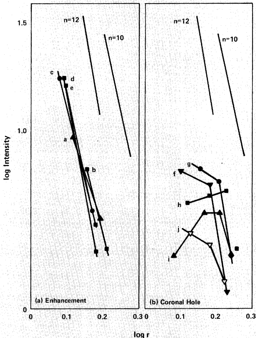
Fig. 20. Emission line intensity versus radial distance for (a) a coronal enhancement and (b) a coronal hole region. Data were obtained during the May 30, 1965, total solar eclipse. Letters label lines through data taken at the same position angle. Curves of 1/r^n ( n = 10 and 12 ) are shown for comparison.
