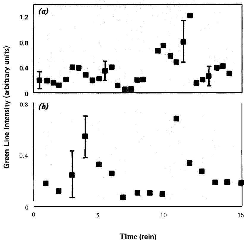
Fig. 17. Peak intensity versus time for two 15-minute segments of Fe XIV emission line data obtained aboard the Concorde 001 at the June 30, 1973, total eclipse. The data in (a), from a region near the base of a helmet streamer at 1.07 R_\odot , suggest intensity variations with a periodicity of about 5 minutes corresponding perhaps to a coronal response to the 5-minute oscillations of the photosphere. Tracking problems introduced the errors shown by the bars. The data in (b) are from an equatorial bright coronal region at 1.07 R_\odot . The sudden intensity increase followed by a slow decay suggests the presence of a shock disturbance. The variations have a periodicity of about 6 minutes.
