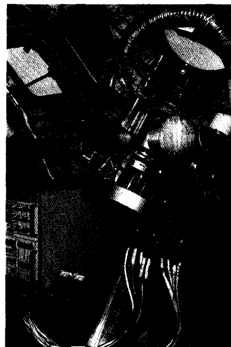
Fig. 10. Los Alamos-designed telescope for photographic polarimetry and electronic control equipment (lower left) mounted in aircraft. This instrument photographs the corona beyond 12 R_\odot and has provided data for determining electron densities and image-enhanced photographs of the outer corona. (See note "Unique Record of the Changing Corona.") The blue cylinder (upper right) is one of three orthogonally mounted gyroscopes obtained from NASA Apollo program. These provide the inertial references that allow this instrument to point at high accuracy even when the aircraft is in motion.
