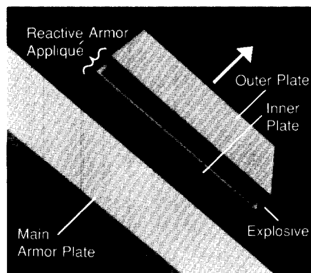
REACTIVE ARMOR
