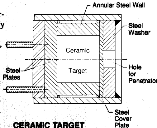
CERAMIC TARGET
