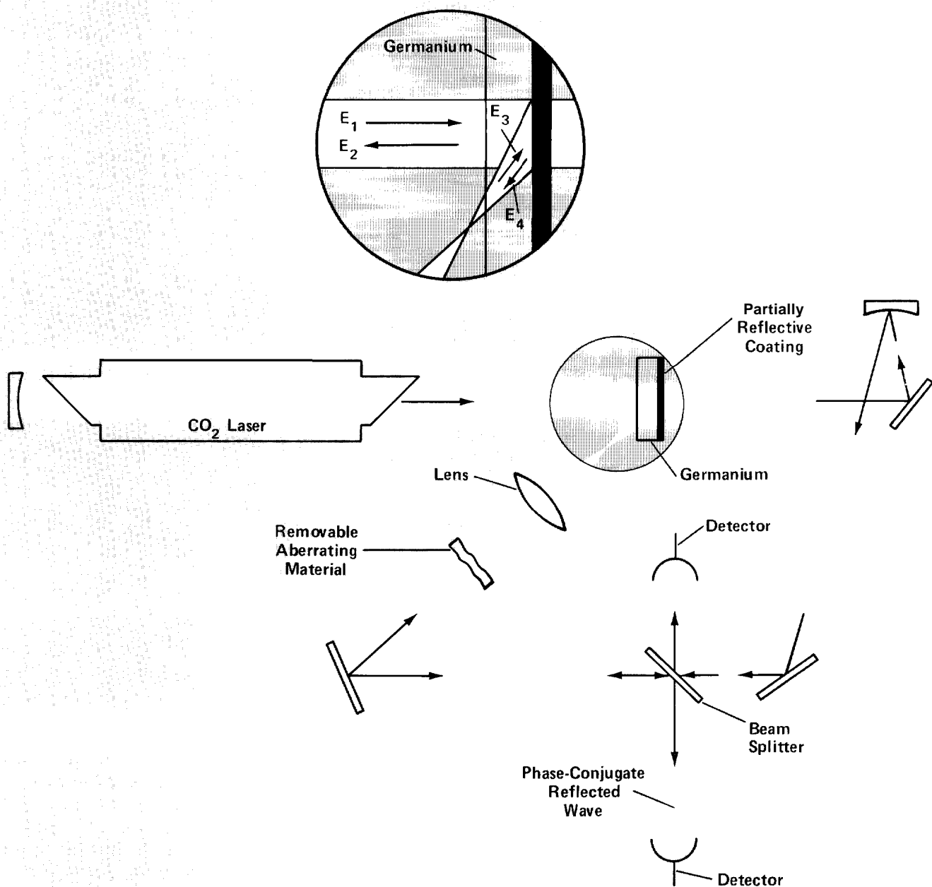
Fig. 10. Degenerate four-wave mixing in the infrared. Here the \text{CO}_2 laser shown in Fig. 9b with counterpropagating fields E_1 and E_2 has part of its output directed at an angle back into the germanium to form the field E_3 . Since this arrangement provides the proper conditions for degenerate four-wave mixing (Fig. 7), the phase-conjugate wave E_4 is generated. The beam
