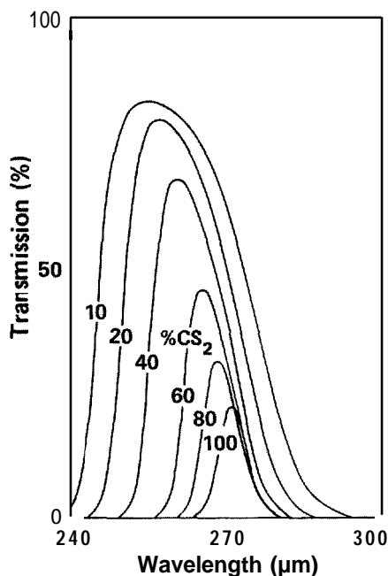
Fig. 13. The transmission spectra of various \text{CS}_2 -hexane solutions. The transmission increases, broadens, and shifts as the percentage of \text{CS}_2 in the mixture decreases. These curves are for 1-millimeter path lengths through the sample.
