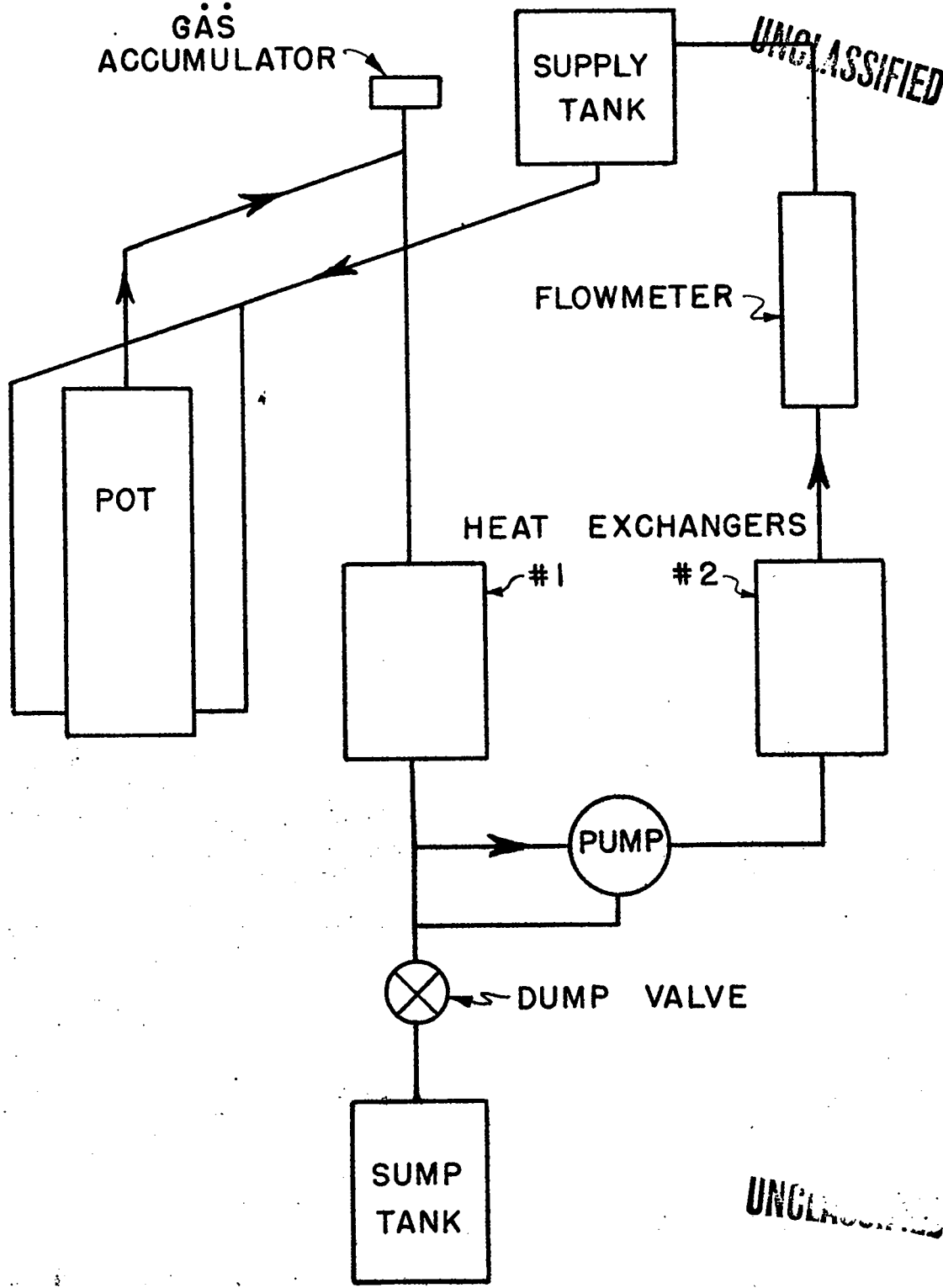
MERCURY FLOW DIAGRAM
