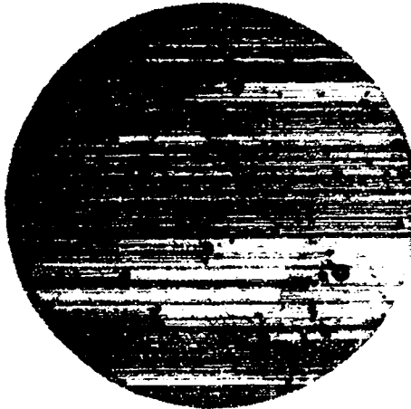
Plate No. J75-A4 Mag.: 250X Chromic acid acetic acid etch; bright field gamma extruded 900°C; extrusion ratio (A/a) 118
