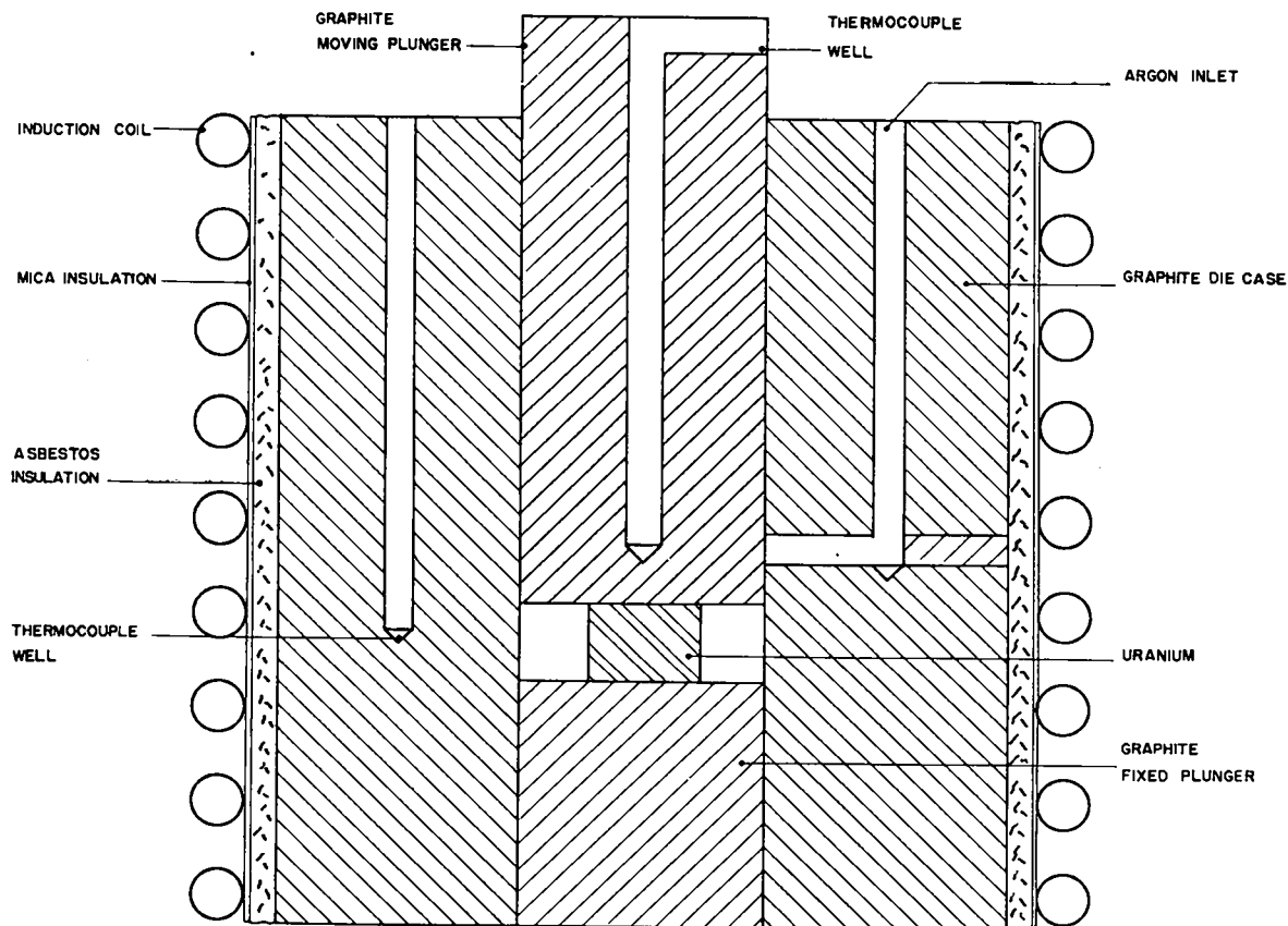
HOT PRESSING DIE ASSEMBLY
