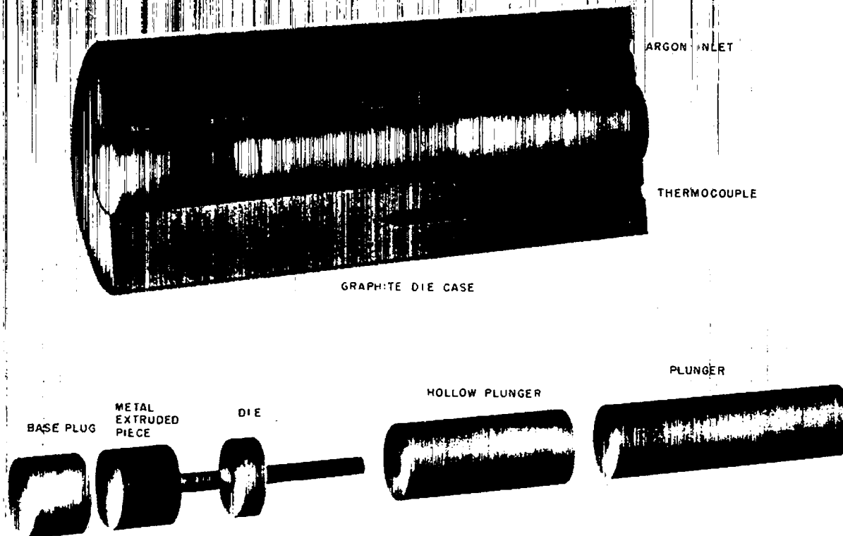
EXPLODED VIEW OF DIE ASSEMBLY AND DIE AS- SEMBLY IN CASE
