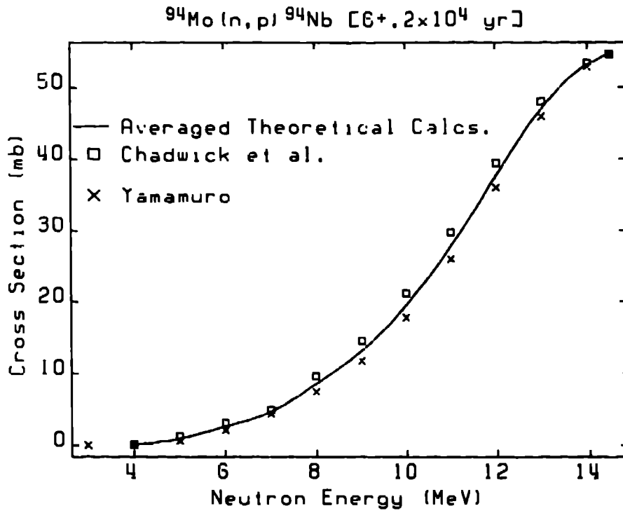
Fig. 1. Theoretical cross sections for (n,p) production of ^{94}\text{Nb} , normalized to a value of 54.5 mb at 14.5 MeV [7].
