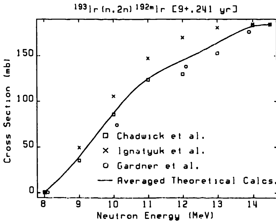
Fig. 8. Theoretical cross sections for (n,2n) production of ^{192m}\text{Ir} , normalized to a value of 184 mb at 14.5 MeV [8].
