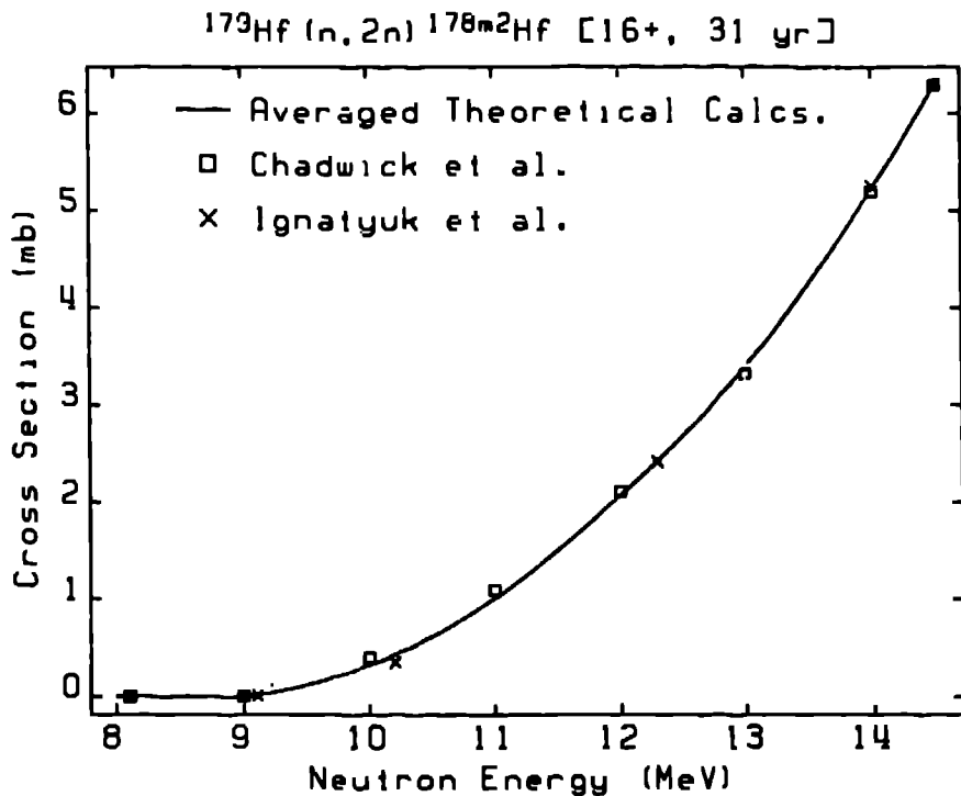
Fig. 7. Theoretical cross sections for (n,2n) production of ^{178}\text{Hf} , normalized to a value of 6.29 mb at 14.5 MeV [7].
