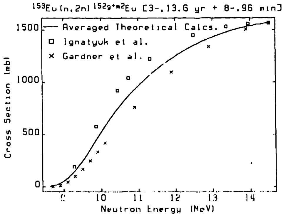
Fig. 4. Theoretical cross sections for (n,2n) production of ^{152\text{g}+\text{m}2}\text{Eu} , normalized to a value of 1568 mb at 14.5 MeV [7].
