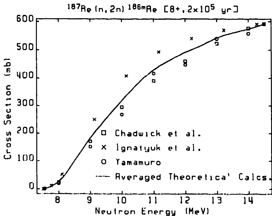
Fig. 6. Theoretical cross sections for (n,2n) production of ^{186m}\text{Re} , normalized to a value of 592 mb at 14.5 MeV [8].
