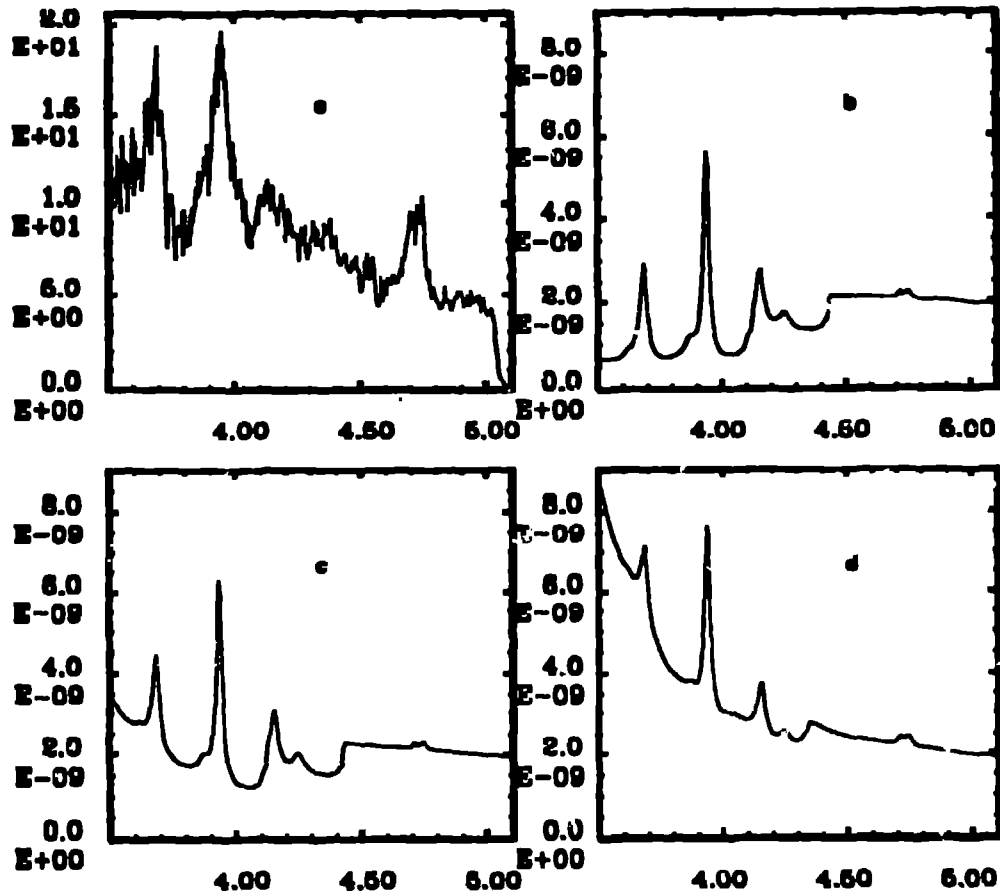
Figure 2. Core-pusher capsule spectra for PS26 pulse shape (X-axis units=keV, Y-axis units=arbitrary) a) Experiment b) Theory-no pusher T_e increase c) Theory-20% uniform pusher T_e increase d) Theory-30% uniform pusher T_e increase
