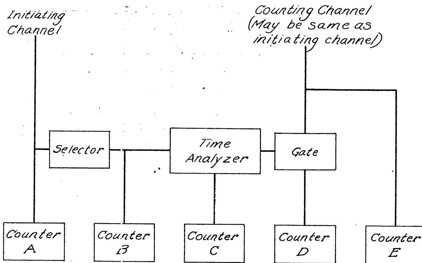
FIG. 1 Block Diagram of Water Boiler Rossi Experimental Apparatus
