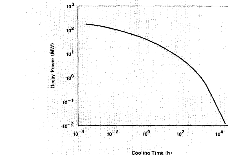
Fig. 7. A log-log plot of decay power as a function of time after reactor scram for the Three Mile Island Unit 2 reactor. This curve was calculated by the Laboratory Nuclear Data Group. It depends on the reactor's power history and fuel and fission-product inventories and on details of the decay chains that fission products and transuranics follow as they spontaneously decay to more stable nuclear states.
