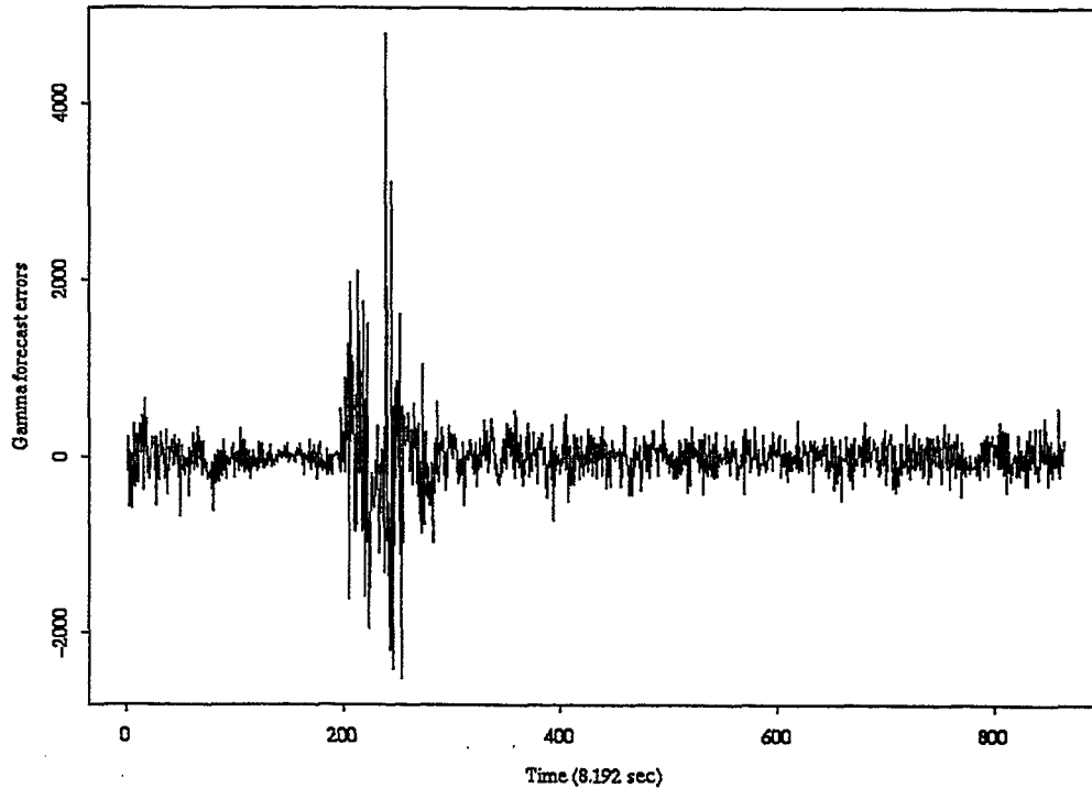
FIGURE 5. The forecast errors that result from a linear model relating gamma counts to electron counts for the region shown in Figs. 3 and 4.
