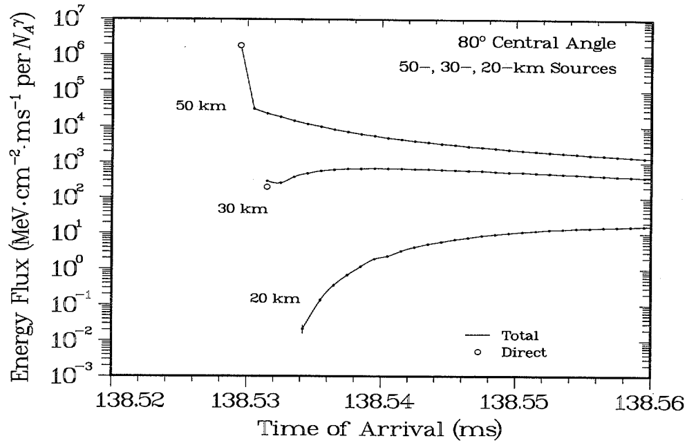
Fig. 3.4a. Expanded view of Fig. 3.3 for sources at a central angle of 80°, showing only the earliest arrival times.
