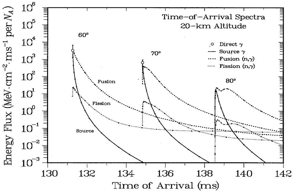
Fig. 5.1b. Energy fluxes as in Fig. 5.1a, but for sources at a 20-km altitude.
