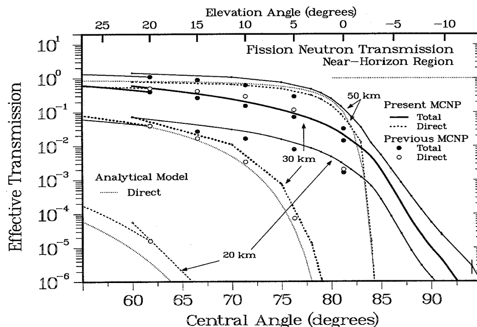
Fig. 4.2b. Angular dependence of the direct and total neutron fluences for fission sources at different altitudes, after integration over both energy and time.
