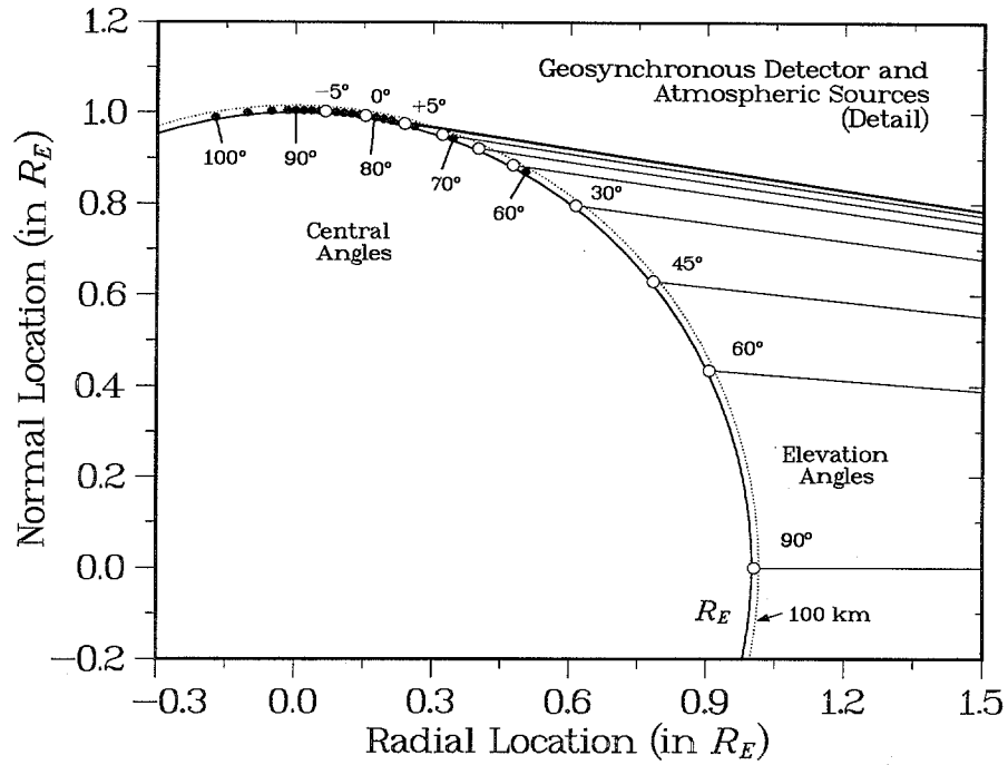
Fig. 2.3b. Enlarged geometry of Fig. 2.3a, emphasizing the connection between source locations, central angles, and elevation angles for a geosynchronous detector orbit. The open circles are sources from Ref. 1 at elevation angles down to \theta = -5^\circ ; the closed circles are sources from the present work at central angles \beta = 60^\circ to 100^\circ .
