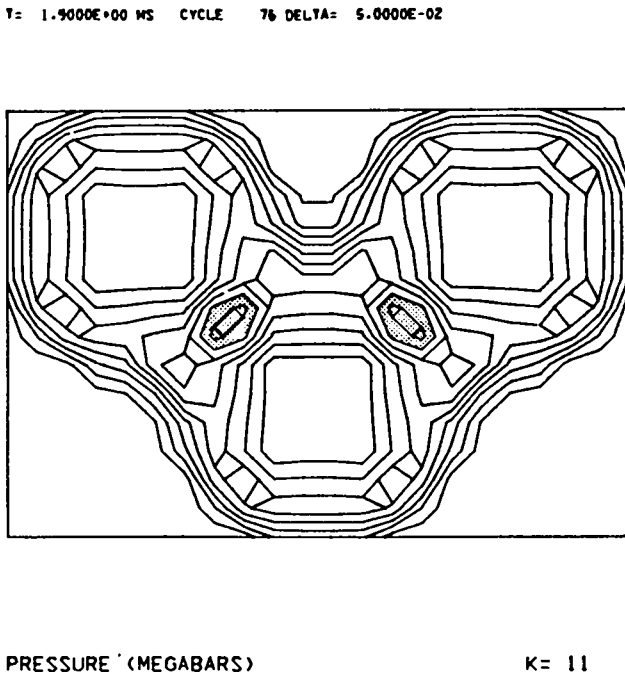
Fig. 10. The nonsymmetric detonator isobar cross section for cell layer k of 11 at 1.90 \mu s. The isobar interval is 50 kbar. The region of double reflection above 400 kbar is shaded.
