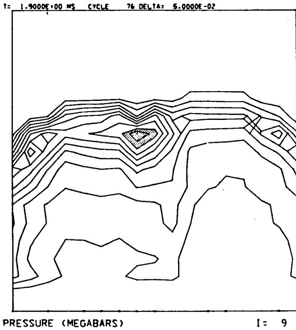
Fig. 9. The symmetric detonator isobar cross section for cell layer i of 9 at 1.90 \mu s. The isobar interval is 50 kbar. The region of triple reflection above 400 kbar is shaded.
