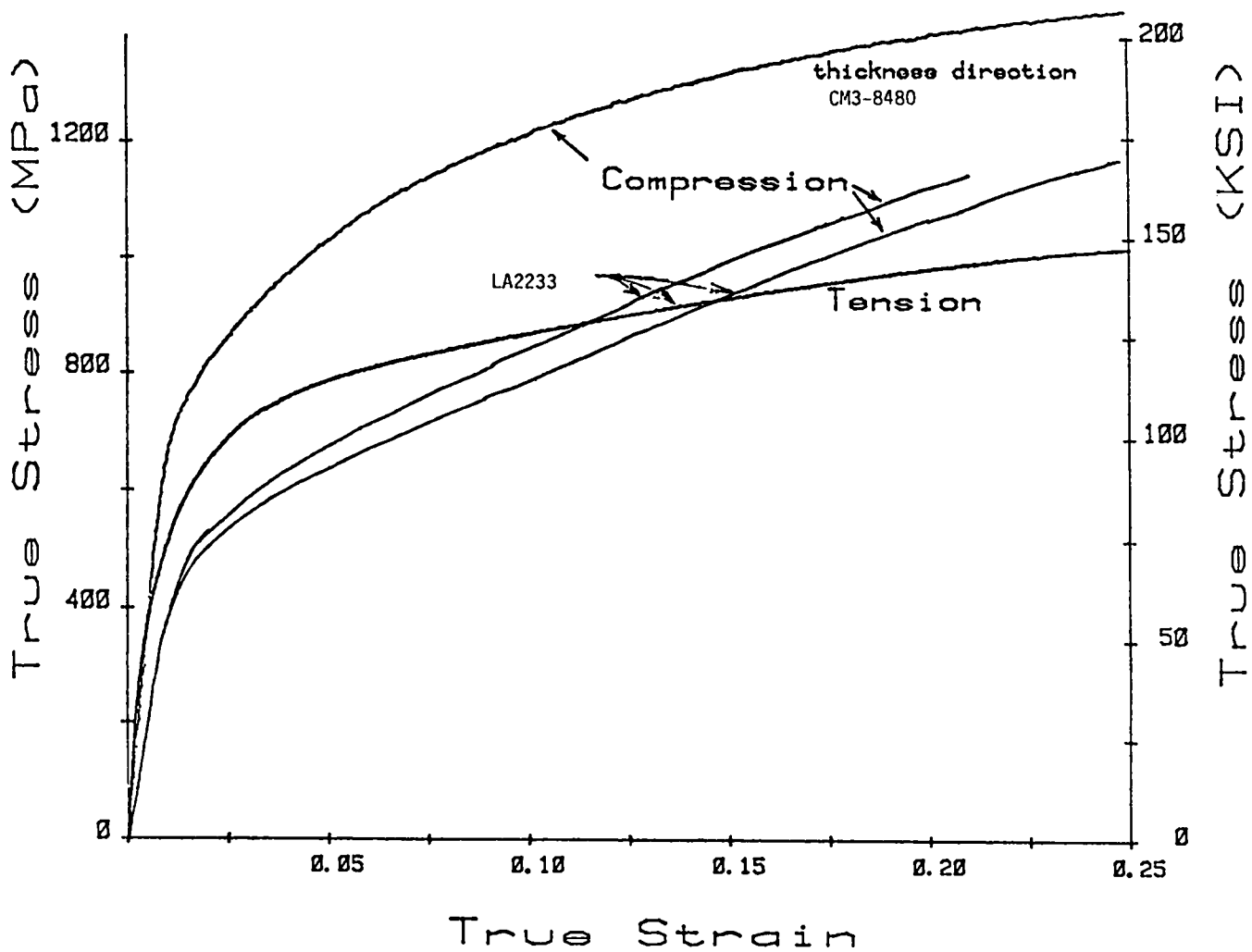
Fig. 10. Comparison of through-thickness CM3-8480 uranium sheet compressive tests to randomly-oriented uranium LA 2233.
