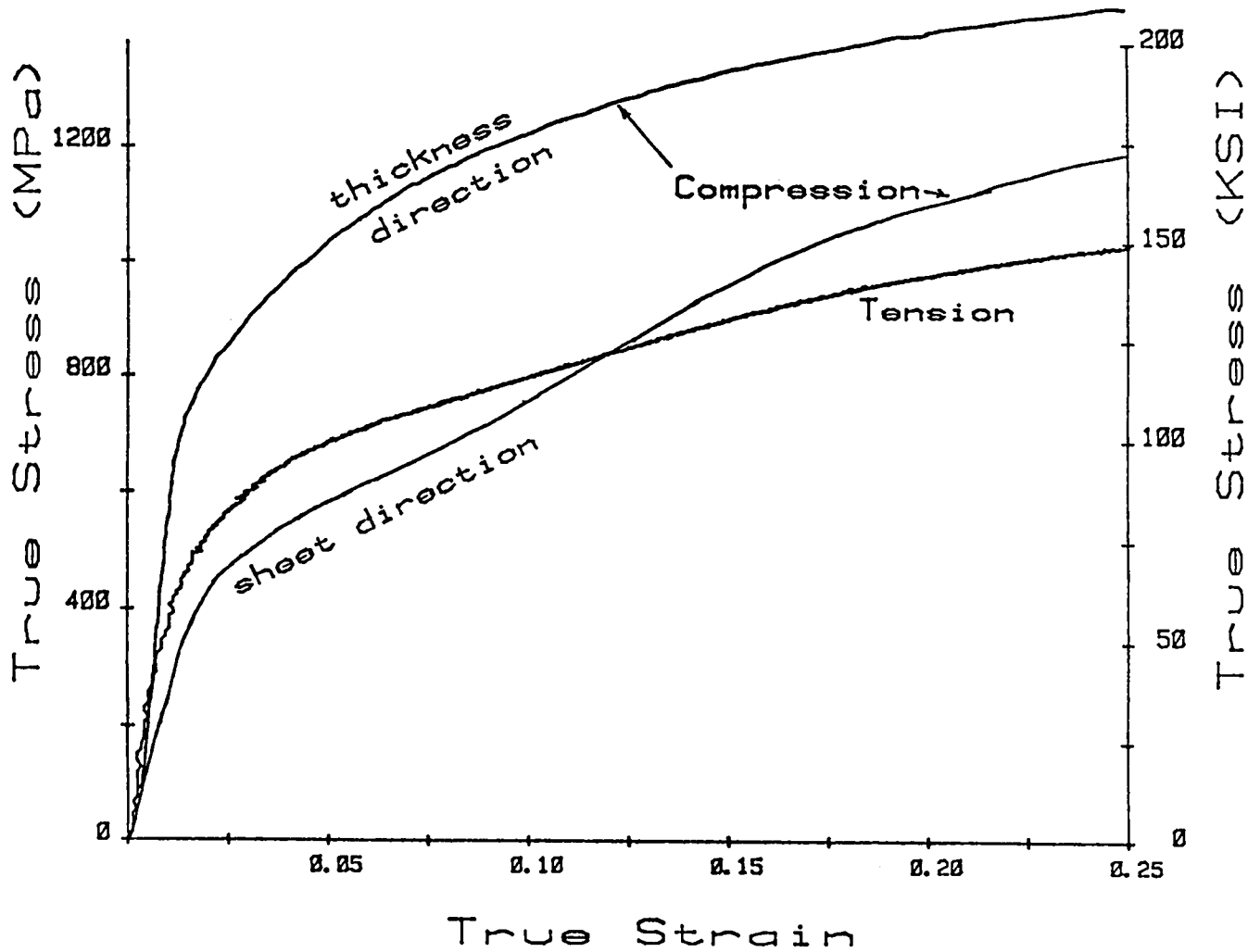
Fig. 8. Comparison of tensile and compressive tests of an unalloyed uranium, CM3-8480, sheet material (Sheet direction "A").
