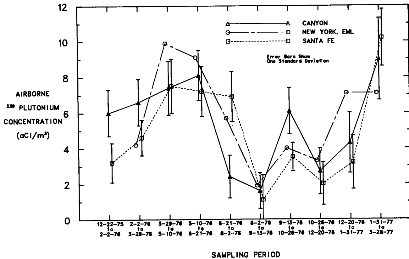
Fig. 18. Concentrations of airborne ^{239}\text{Pu} at three locations during 1976-1977.
