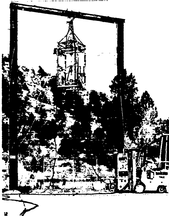
Fig. 10. Lady Godiva suspended outdoors to eliminate the effect of room-return neutrons.
