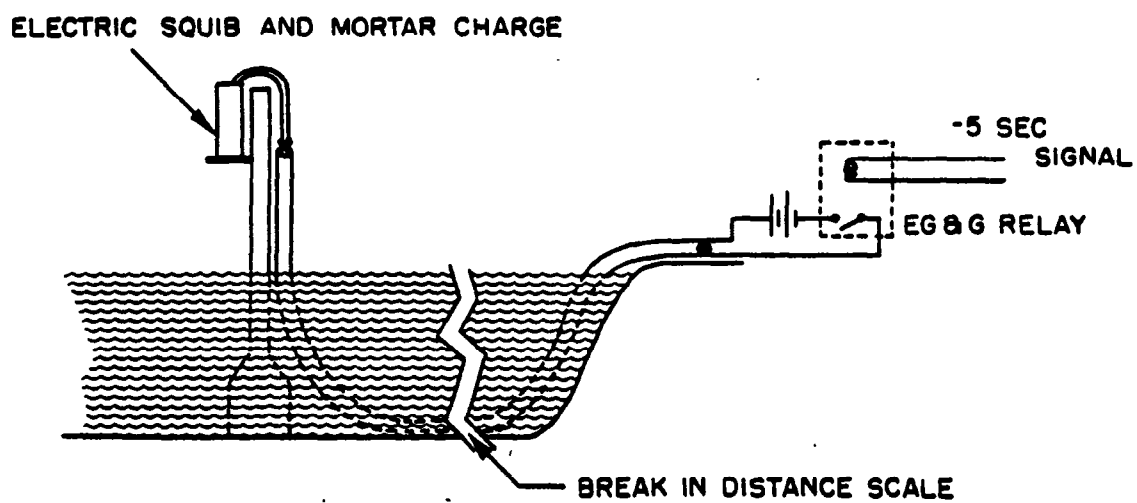
Fig. 2.2—Reef mortar firing system.
