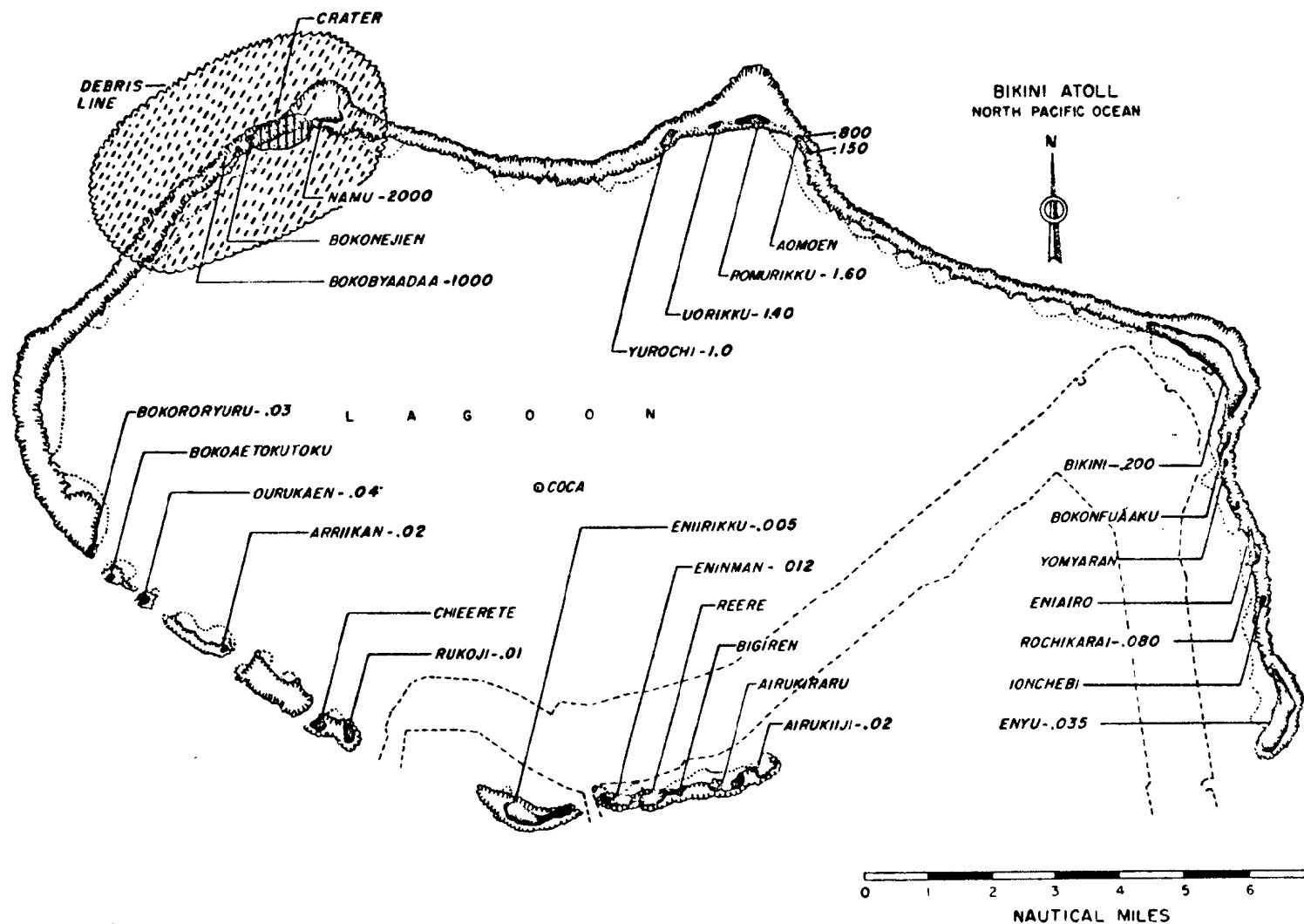
Fig. 4.2— Romeo radiation intensities in roentgens per hour extrapolated to H + 4 hr. Location, barge in crater of Yield, 11 Mt Time fired, 27/0630M March 1954.
