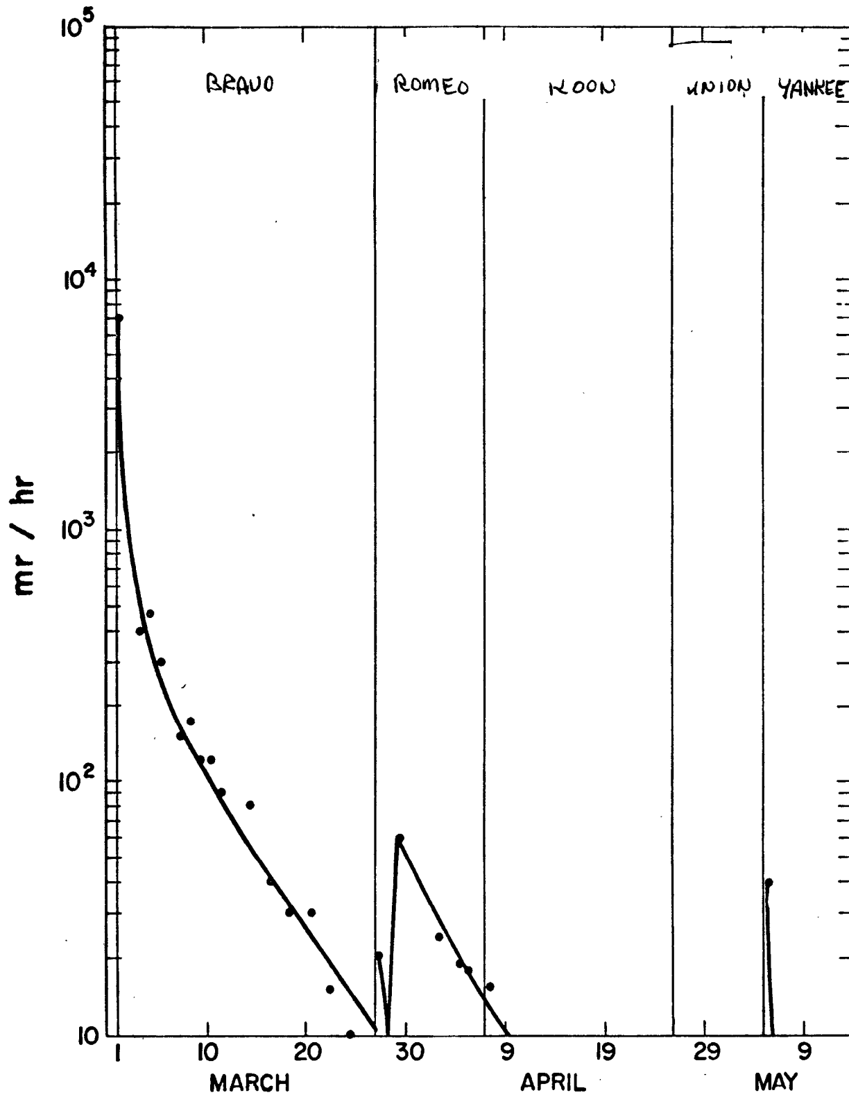
Fig. 4.8—Fall-out record, Airukilji.
