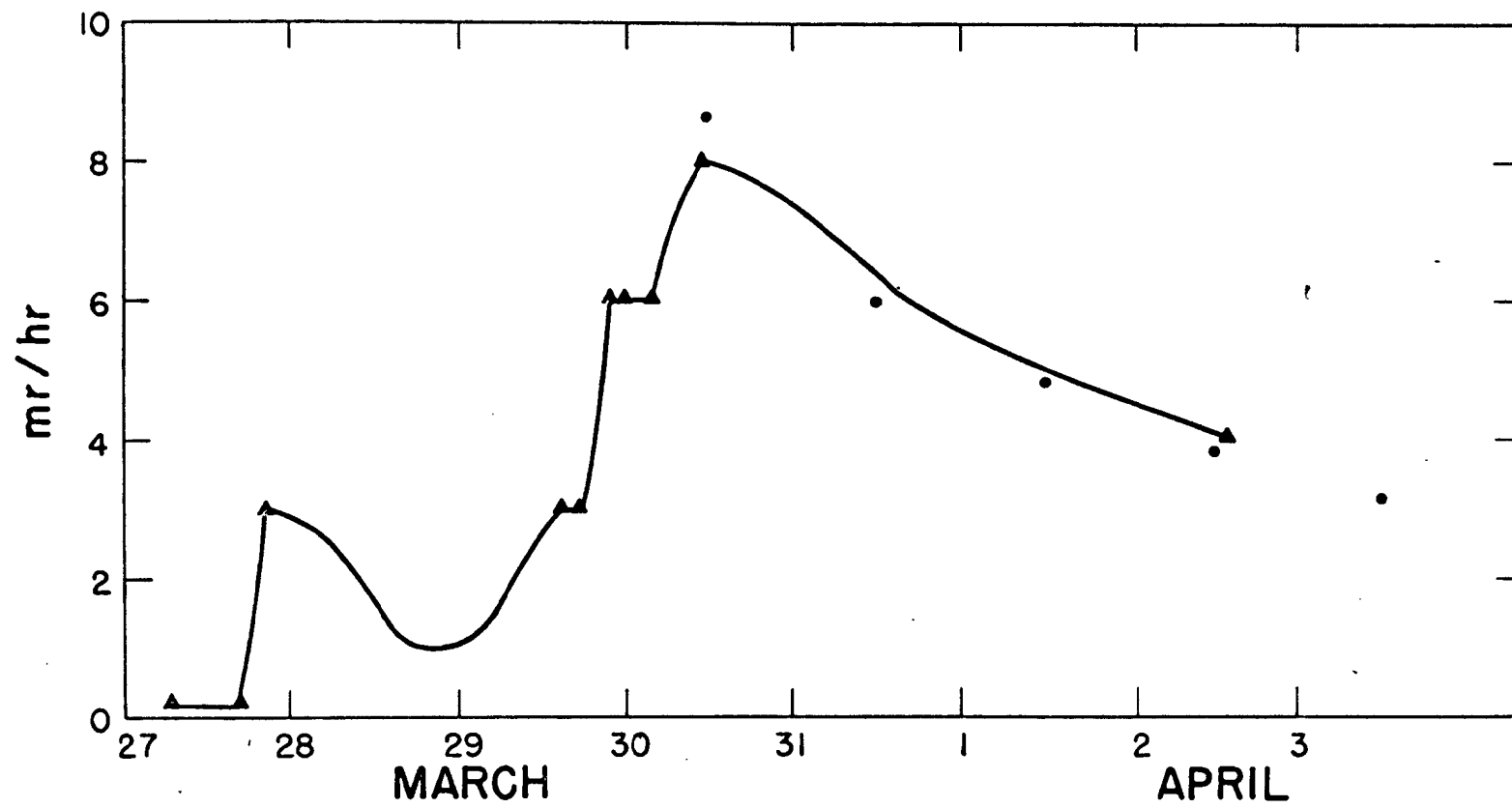
Fig. 4.9 ROMEO radiation fall-out, Parry Island.
