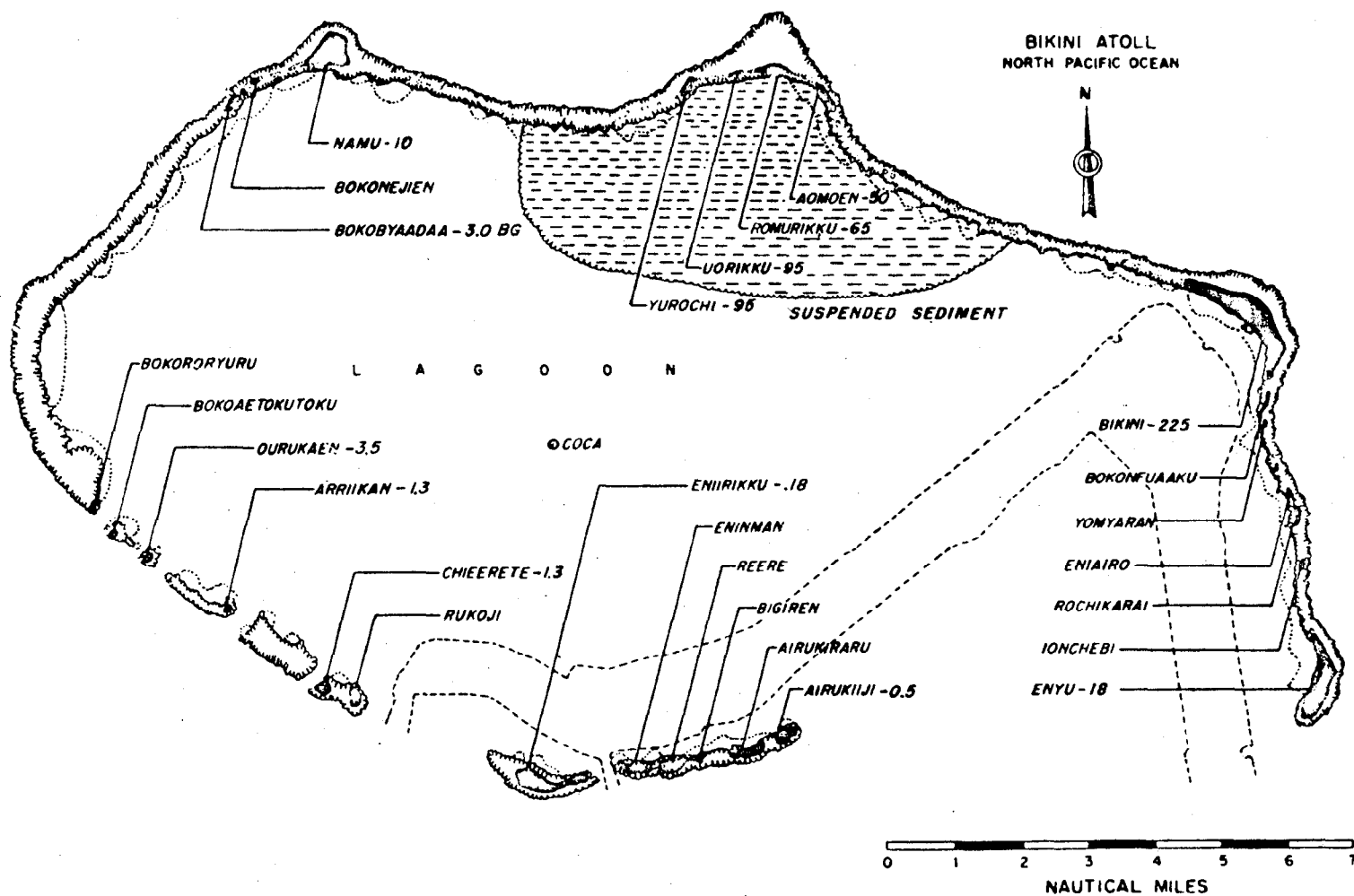
YANKEE Fig. 4.12- radiation intensities in roentgens per hour extrapolated to H+4 hr, plus background (bg) for Bokobyadaa. Location, YANKEE anchorage (barge). Yield, 14 Mt } Time fired, 05/0610M May 1954.
