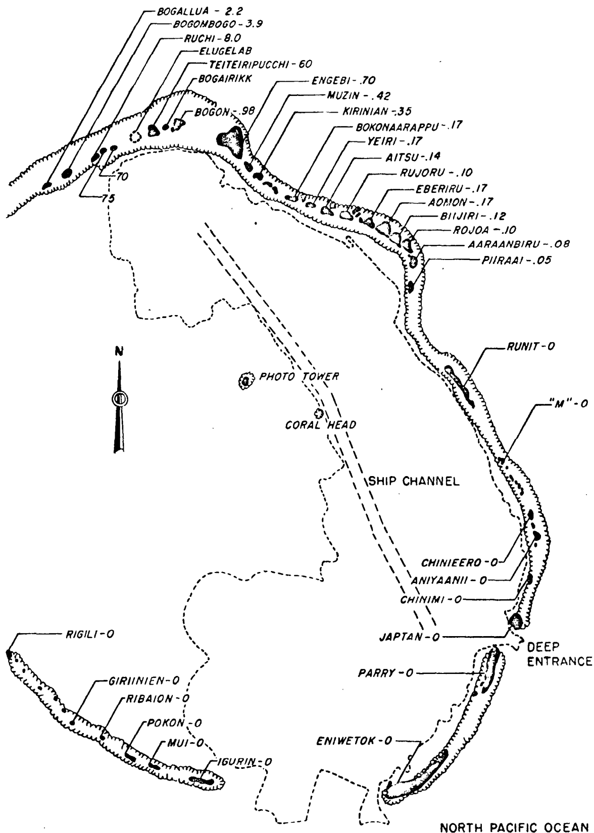
Fig. 4.13 NECTAR radiation intensities in roentgens per hour extrapolated to H + 4 hr. Location, Elugelab crater (barge). Yield, 1.7 Mt. Time fired, 14/0620M May 1954.
