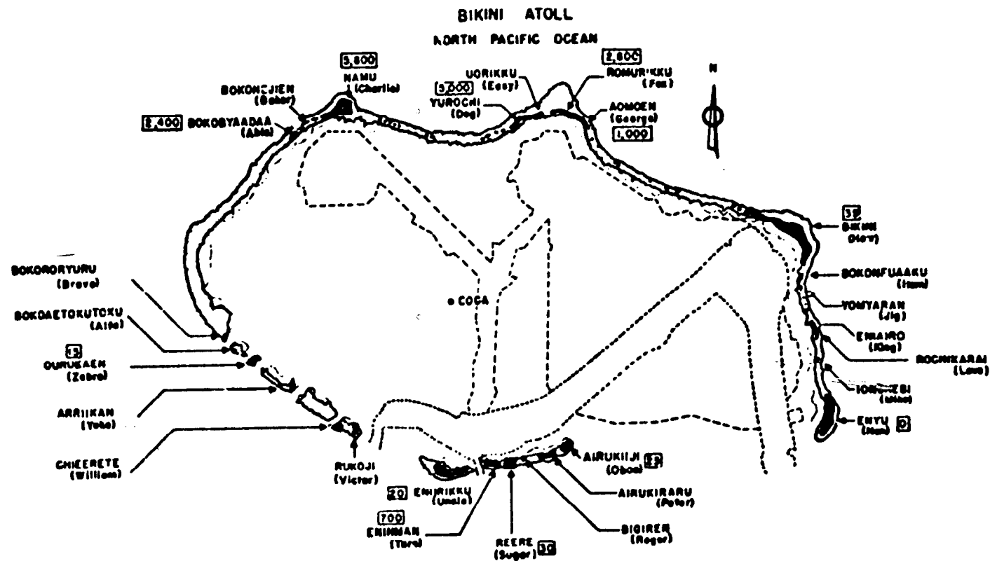
Fig. 3.3- 7 Dakota radiation intensities on Bikini Atoll at H+4 hr. in milliroentgens per hour. Shot site was barge off Yurochi.
